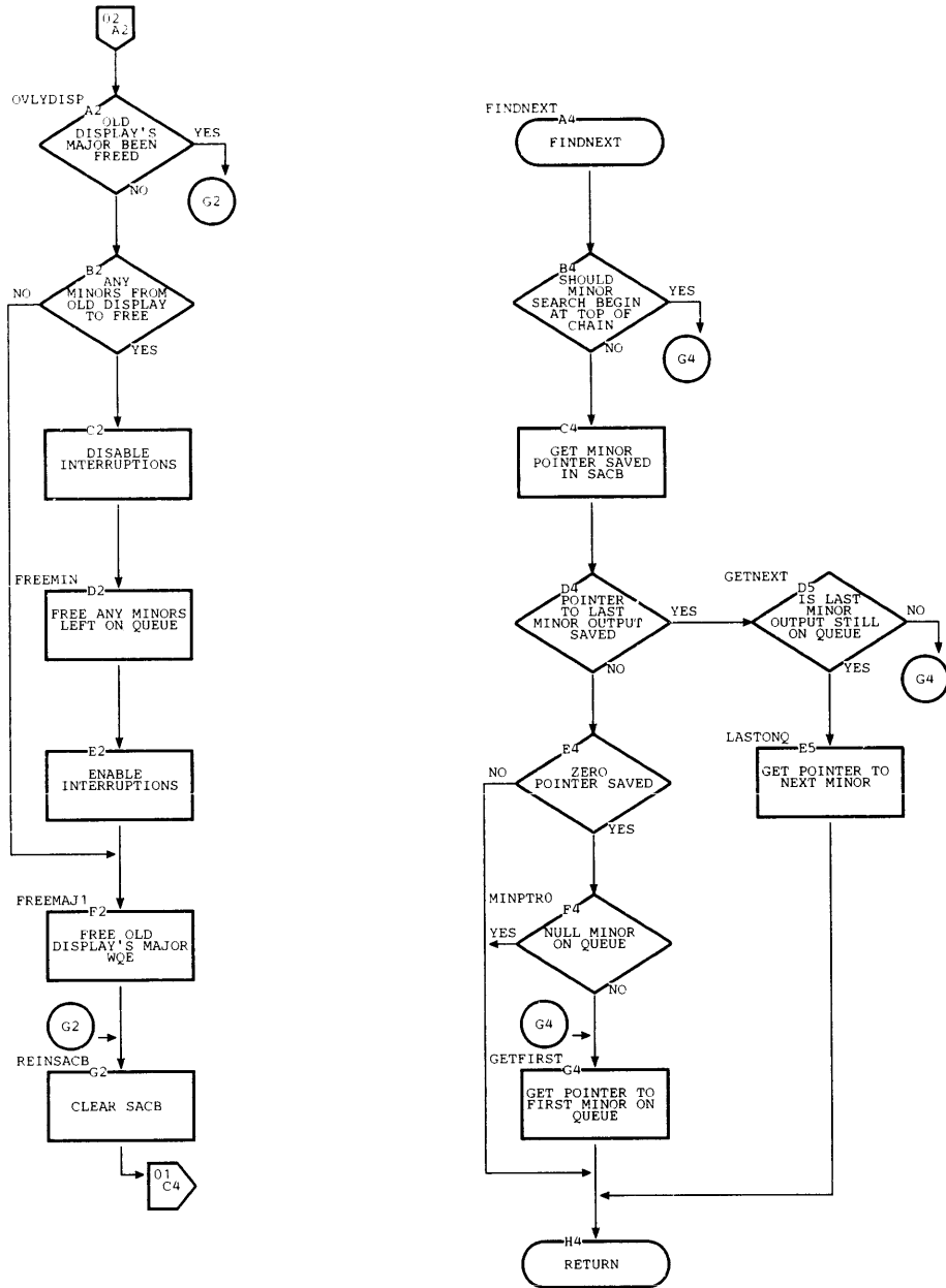
Chart IK. Status Display Interface 2 Routine (Page 2 of 2)
