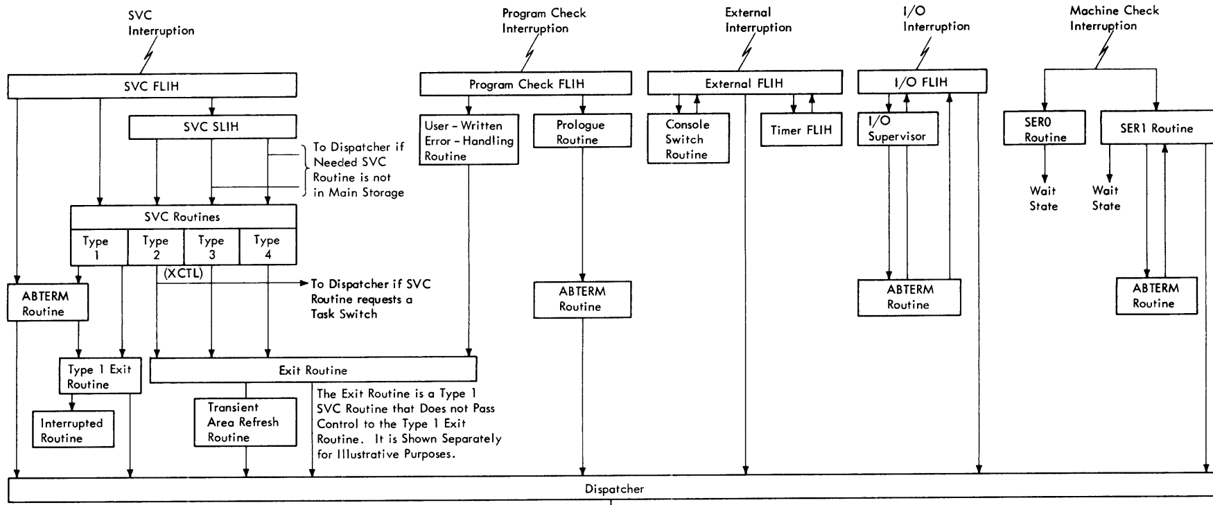
Chart 00. Overall Control Flow of MVT Supervisor
