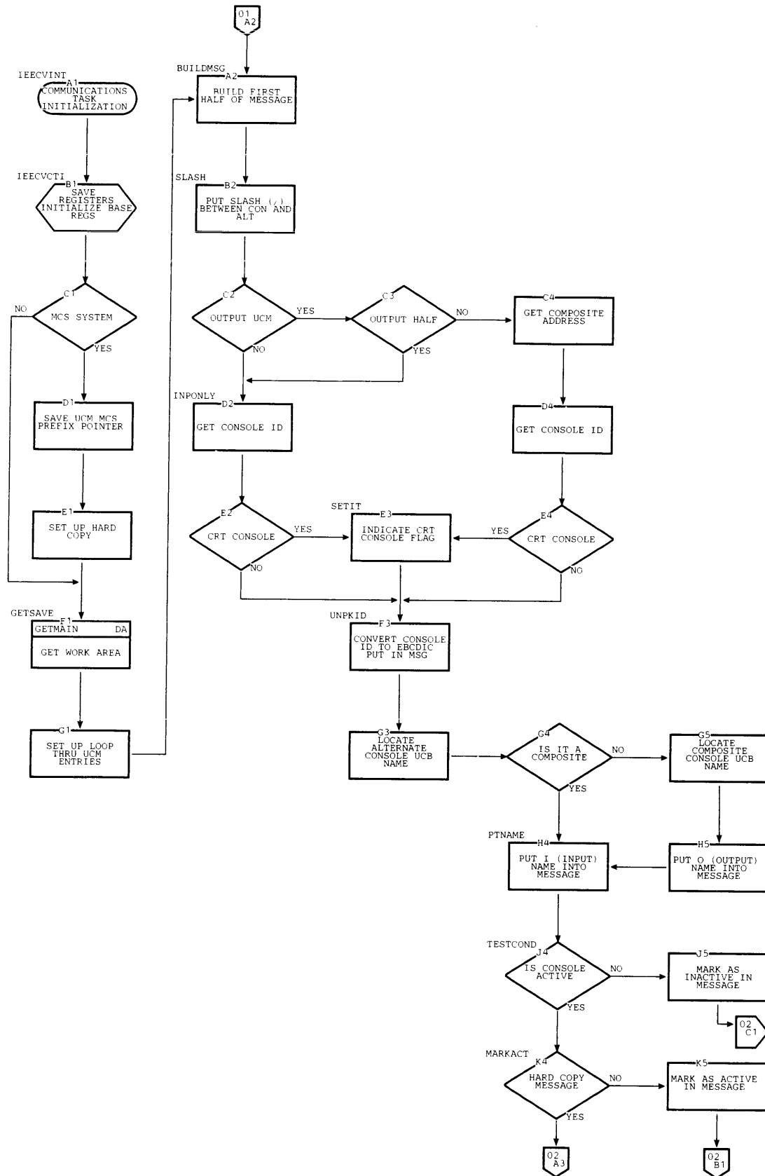
Chart FD. Communications Task Initialization Routine (Page 1 of 5)
