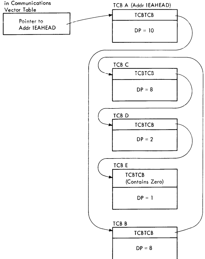
Figure 3-4. The Task Control Block Queue
