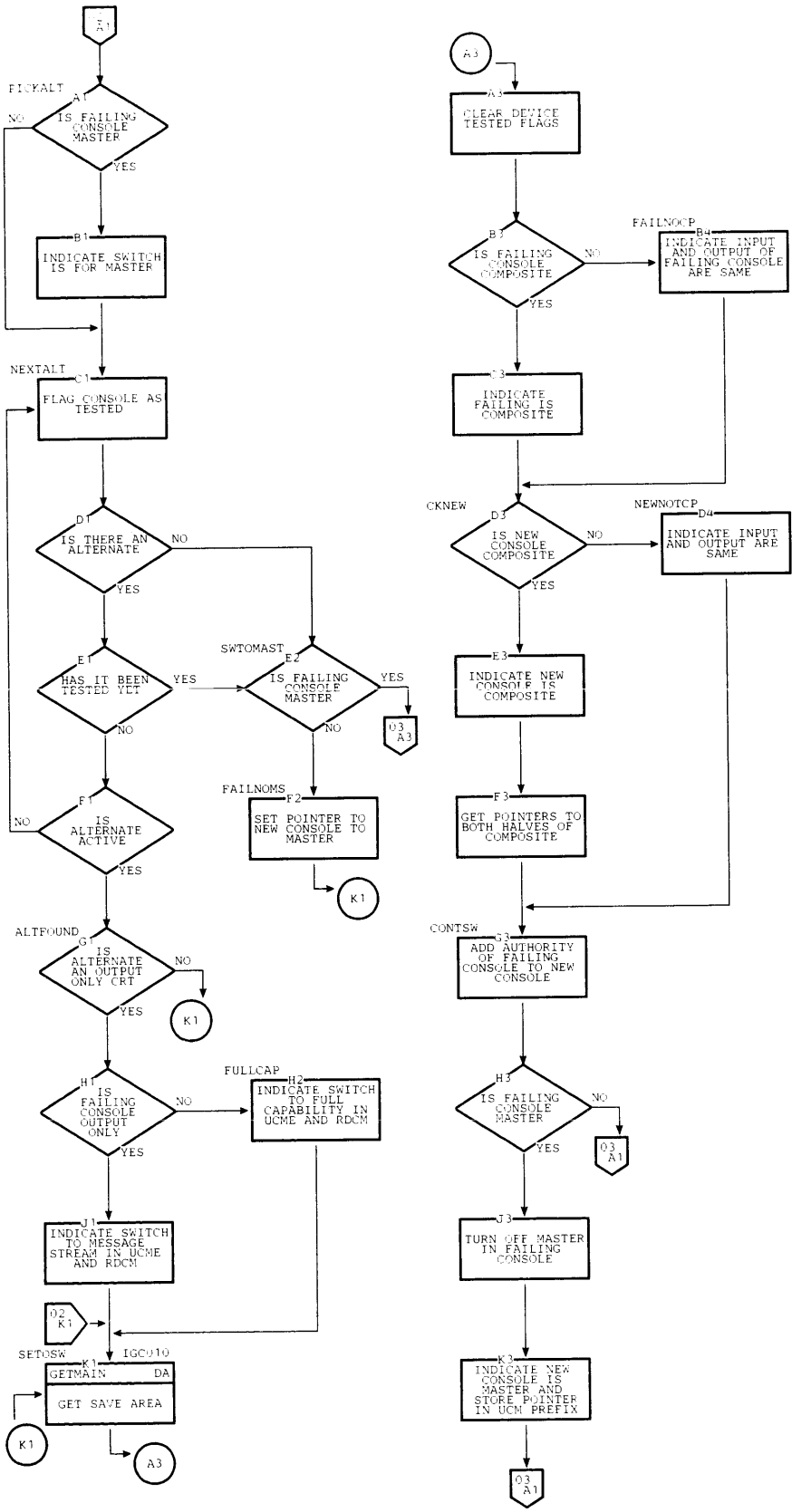
Chart FJ. Console Switch Load 1 -- Communications Task with Multiple Console Support (Page 2 of 3)
