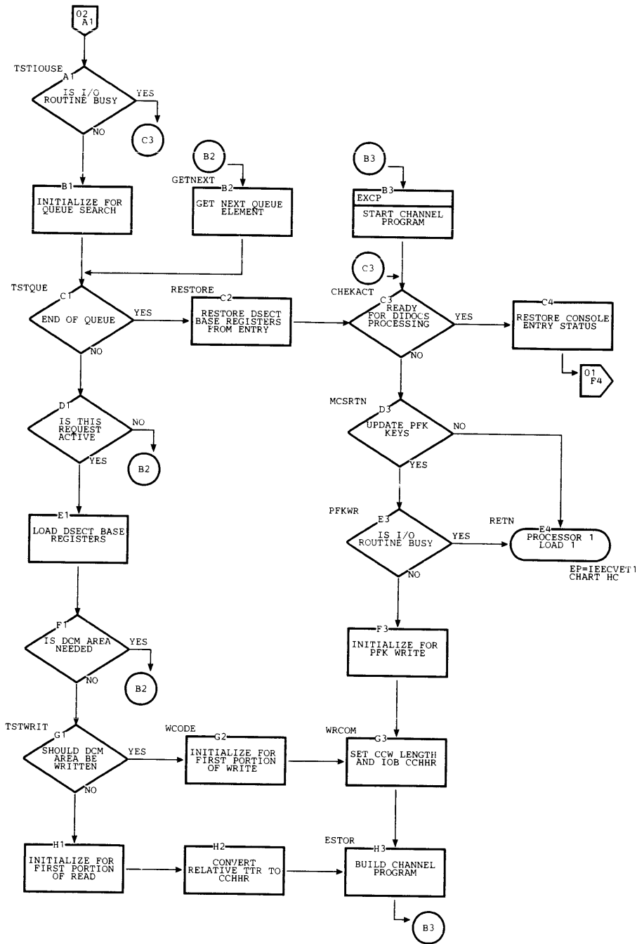
Chart HA. DIDOCs Processor 0, Load 1 (Page 2 of 2)
