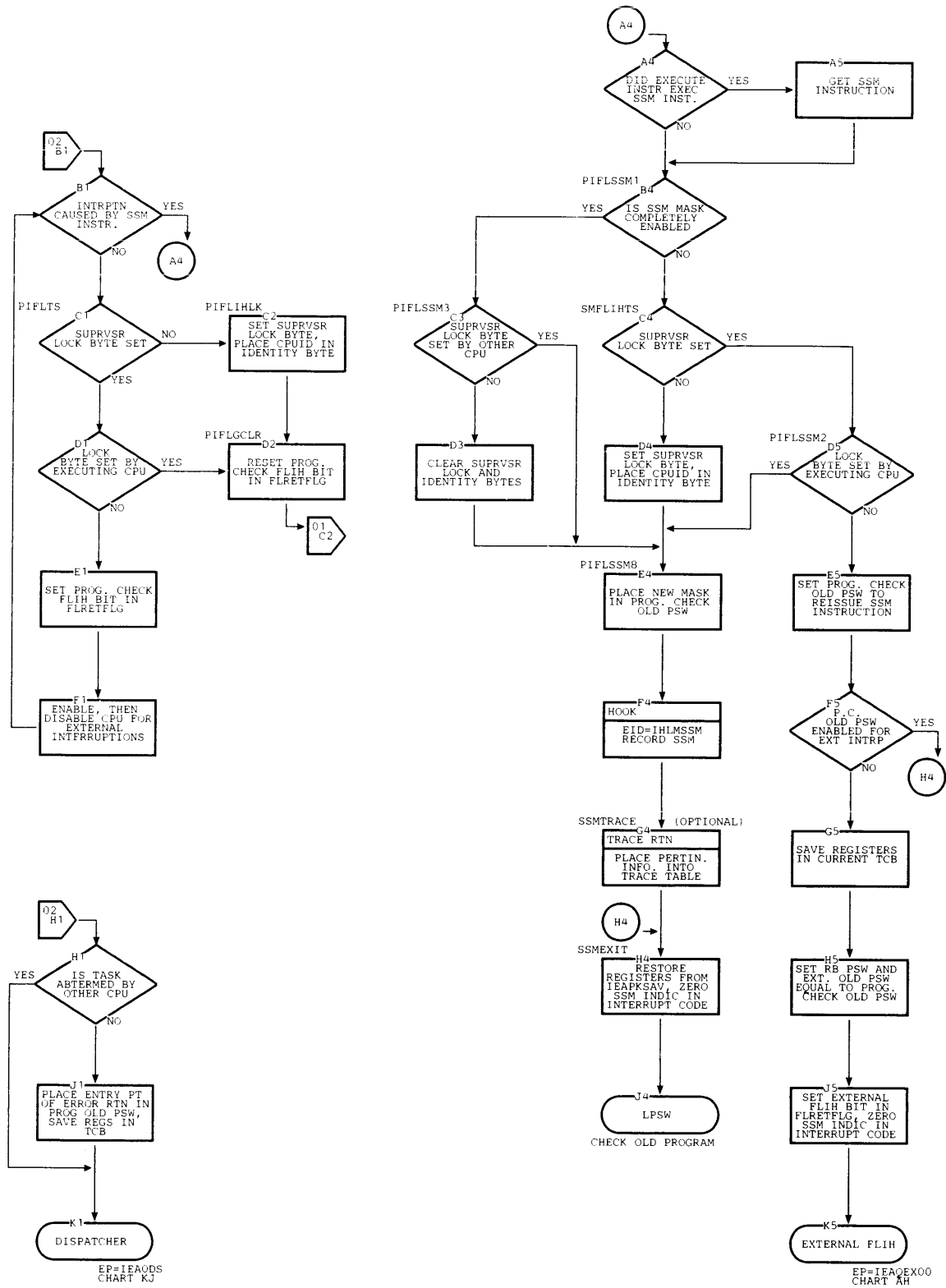
Chart AF. Program Check First-Level Interruption Handler -- Multiprocessing (Page 2 of 2)
