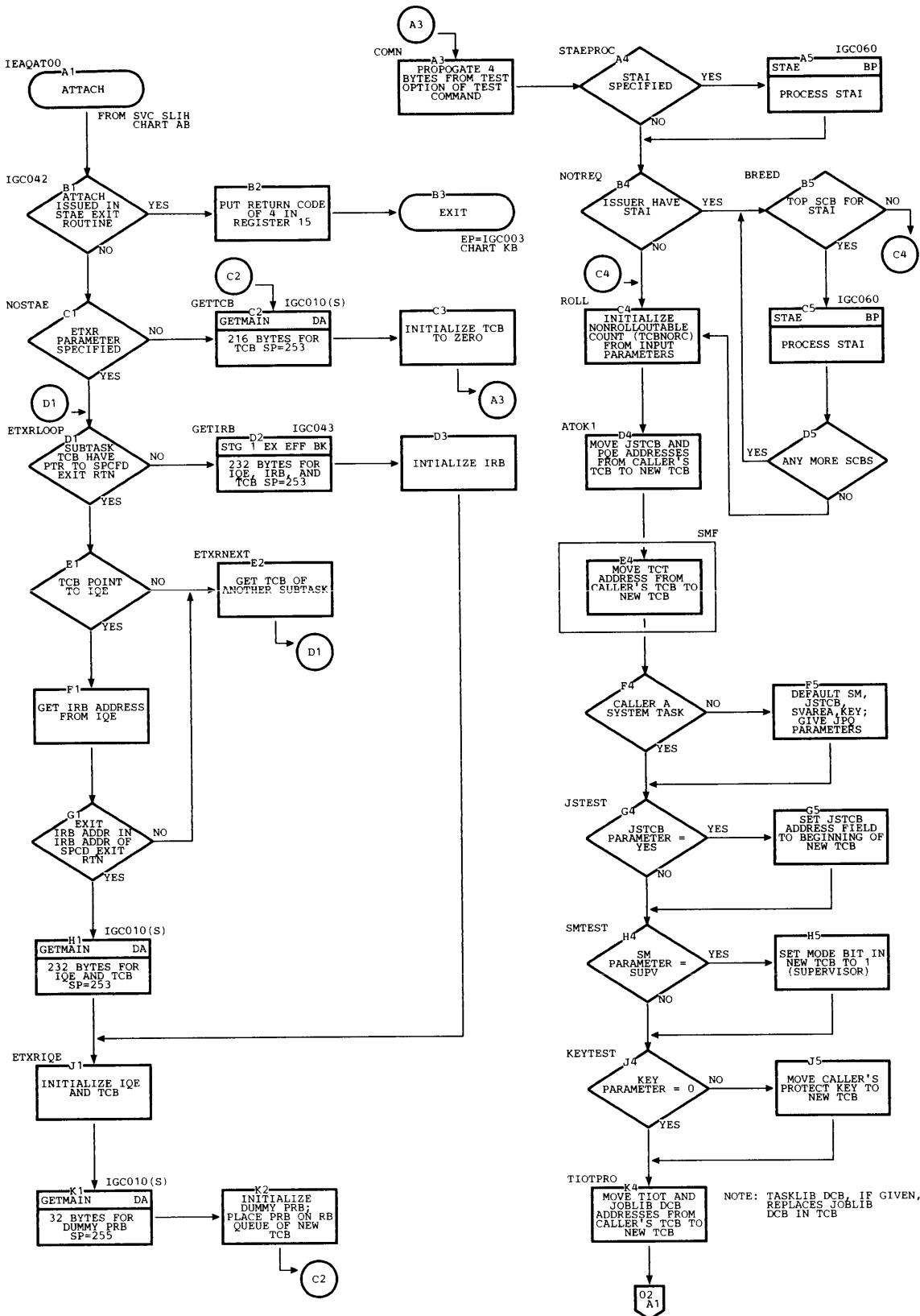
Chart BA. Attach Routine (Page 1 of 4)
