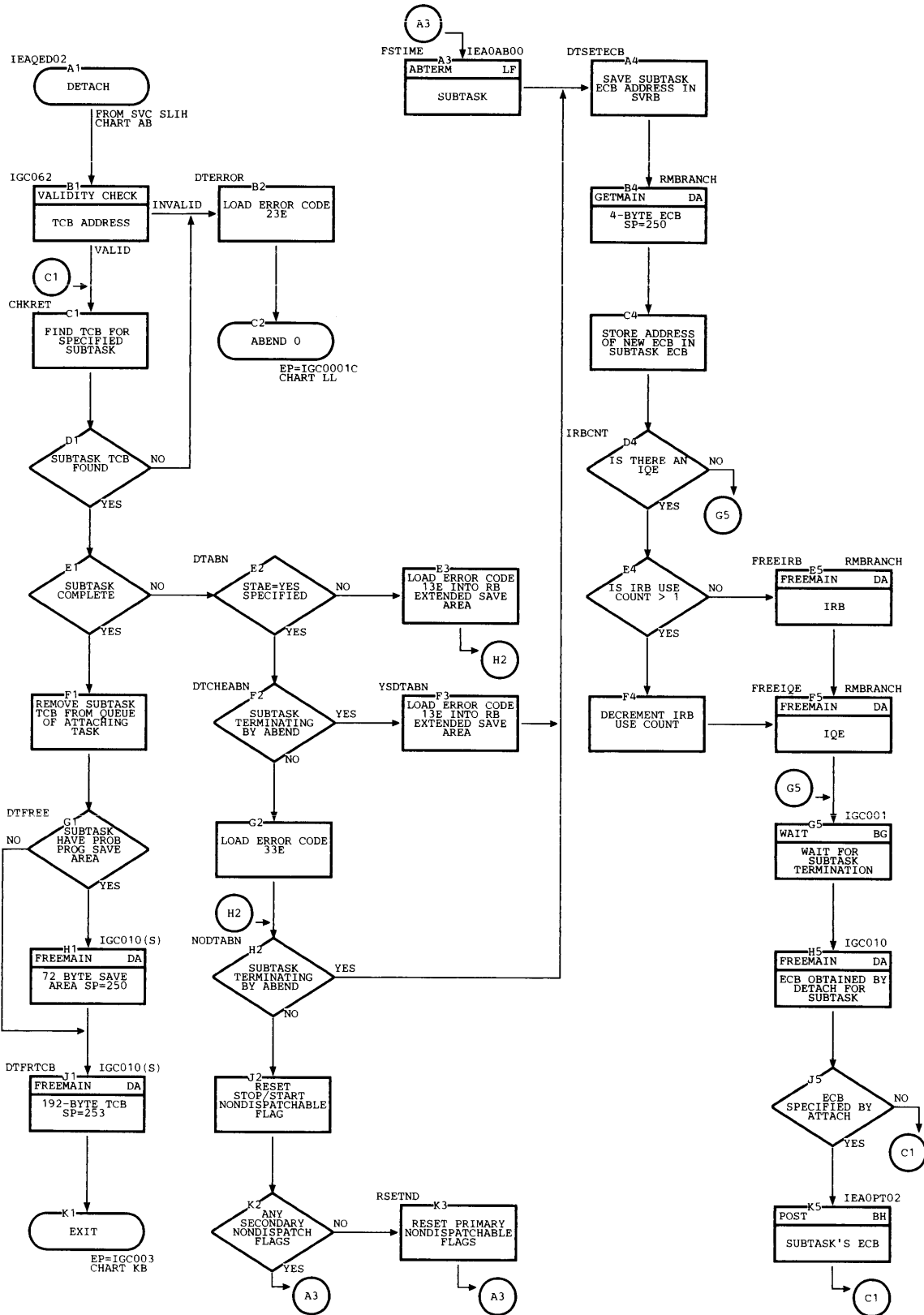
Chart BE. Detach Routine
