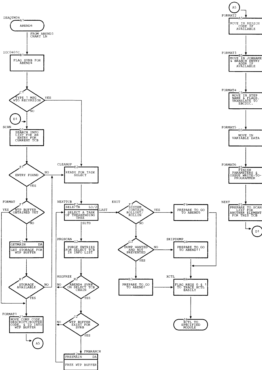
Chart 10. ABEND4 (Page 1 of 2)
