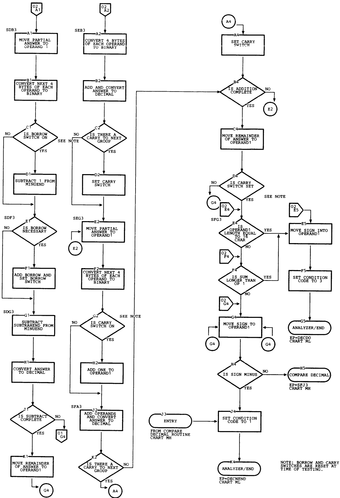
Chart MI. Model 91 Add/Subtract/Zero-and-Add Decimal Routine (Page 2 of 2)
