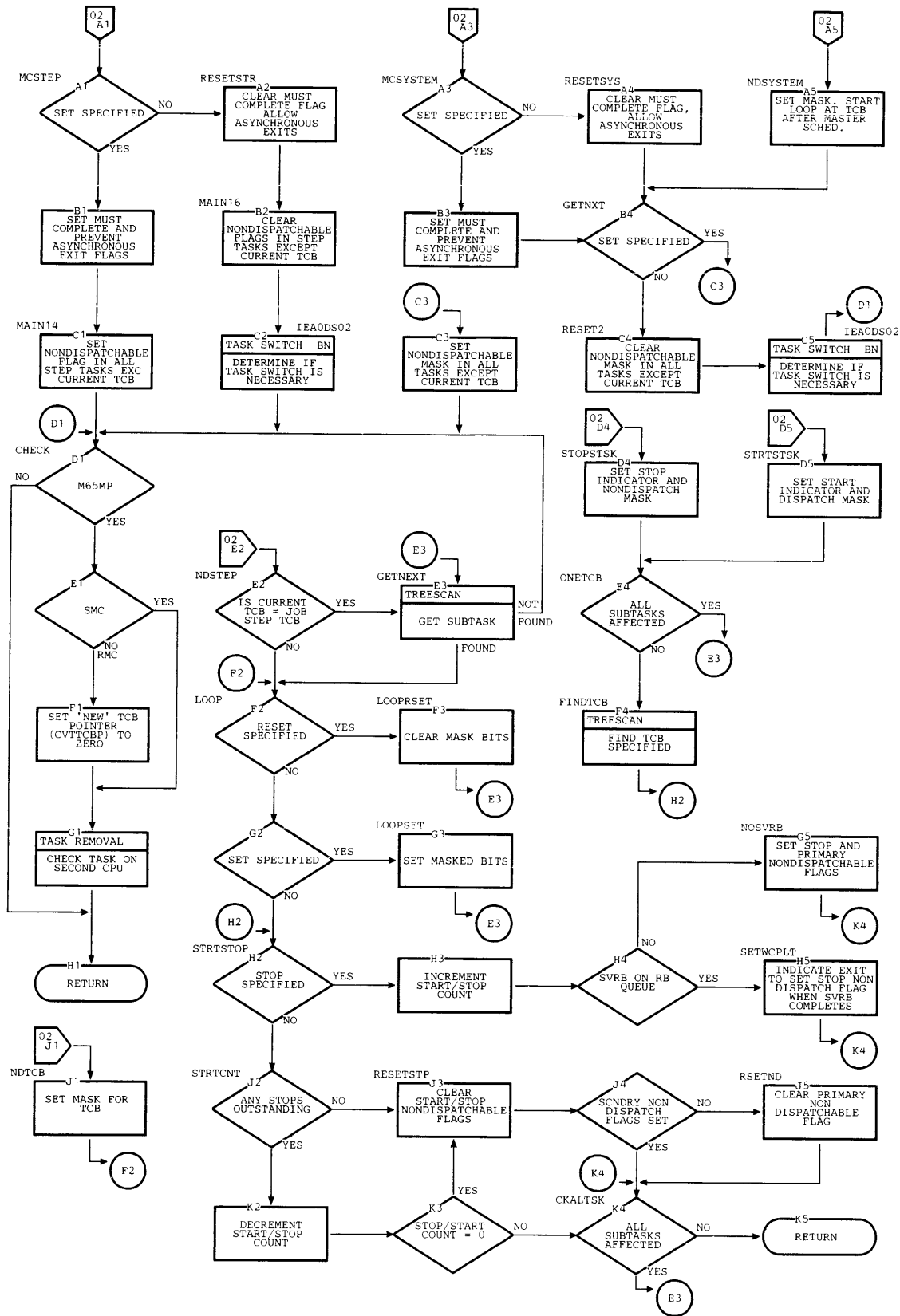
Chart BW. Set Status Service Routine (Page 2 of 2)
