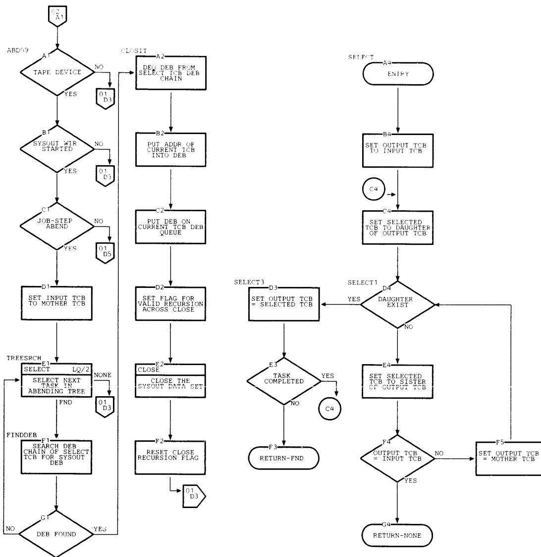
Chart LQ. ABEND7 (Page 2 of 2)
