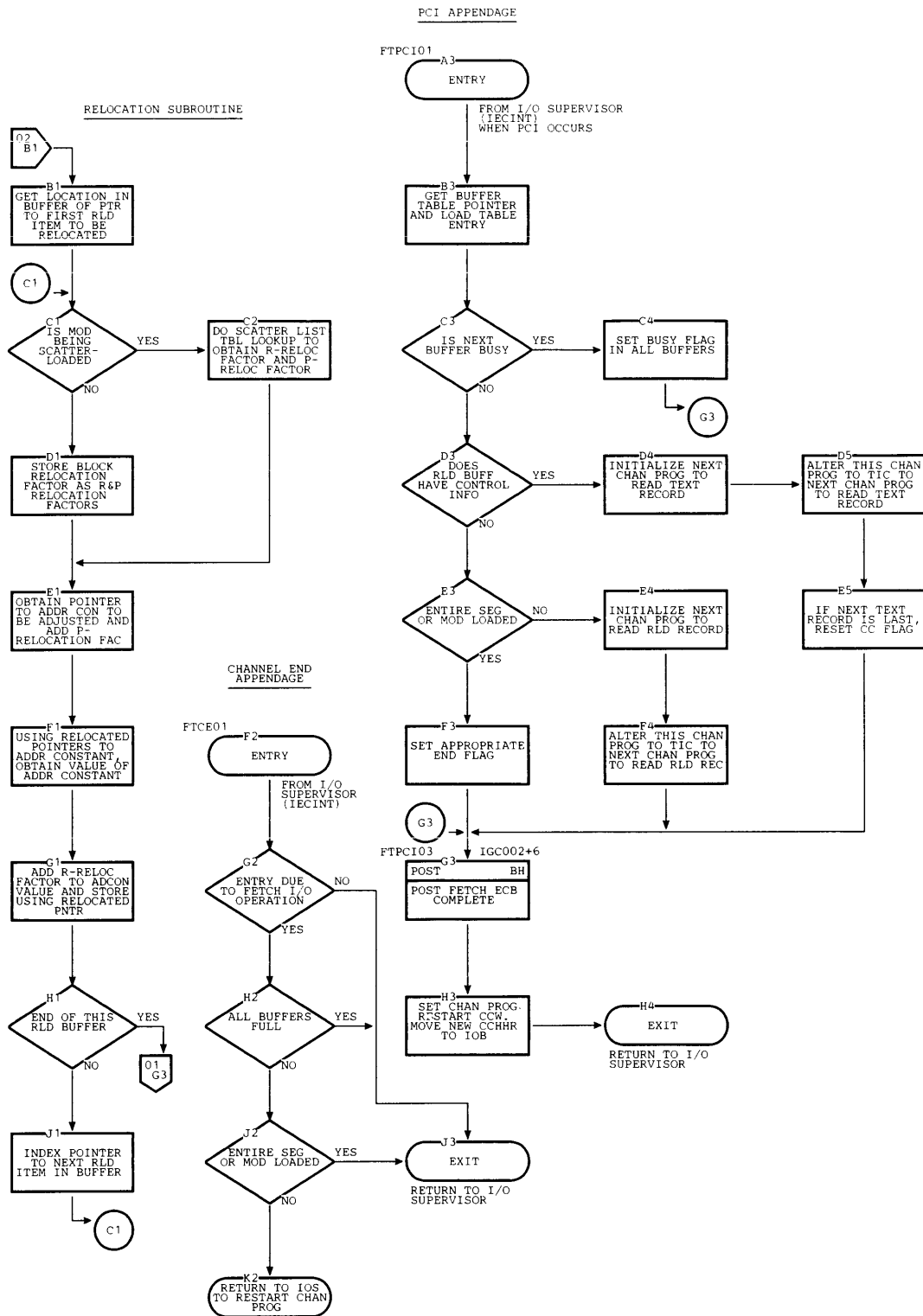
Chart CD. Program Fetch Routine -- PCI and Channel End Appendages (Page 2 of 3)
