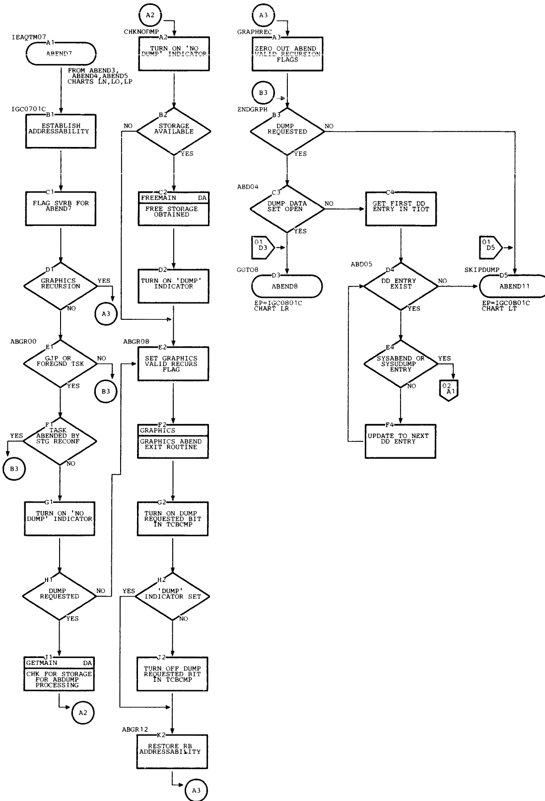
Chart IQ. ABEND7 (Page 1 of 2)
