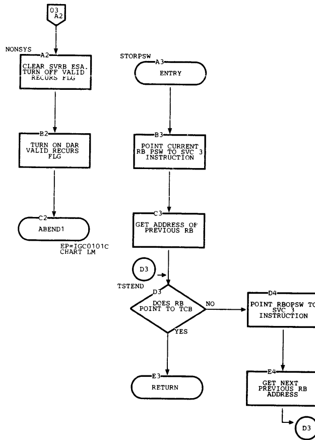
Chart MC. DAR3 (Page 3 of 3)
