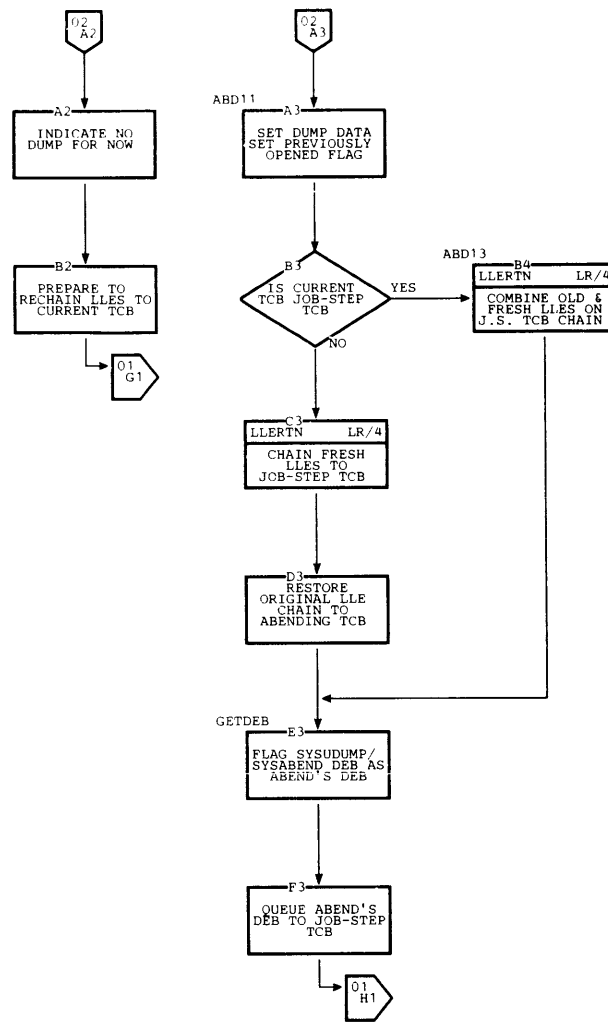
Chart LR. ABEND8 (Page 2 of 4)
