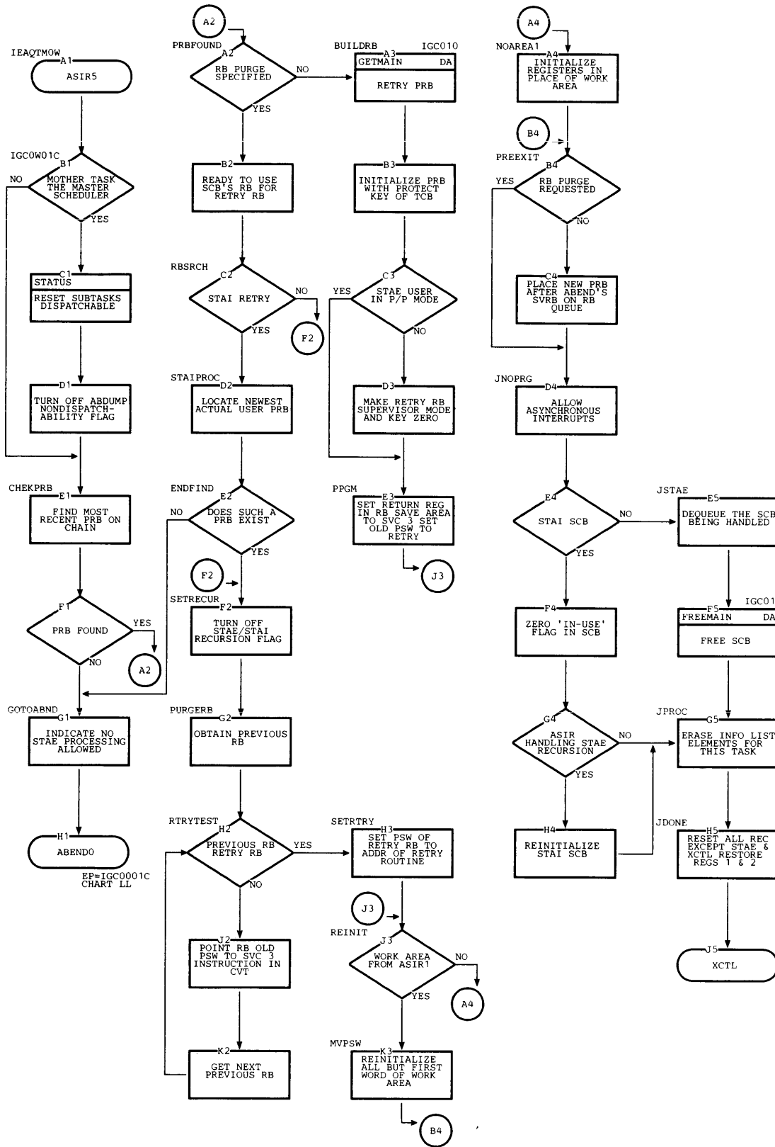
Chart EV. ABEND/STAE Interface 5 Routine (ASIR5)
