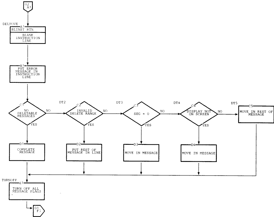
Chart HM. DIDOCS Message 2 Routine (Page 2 of 2)
