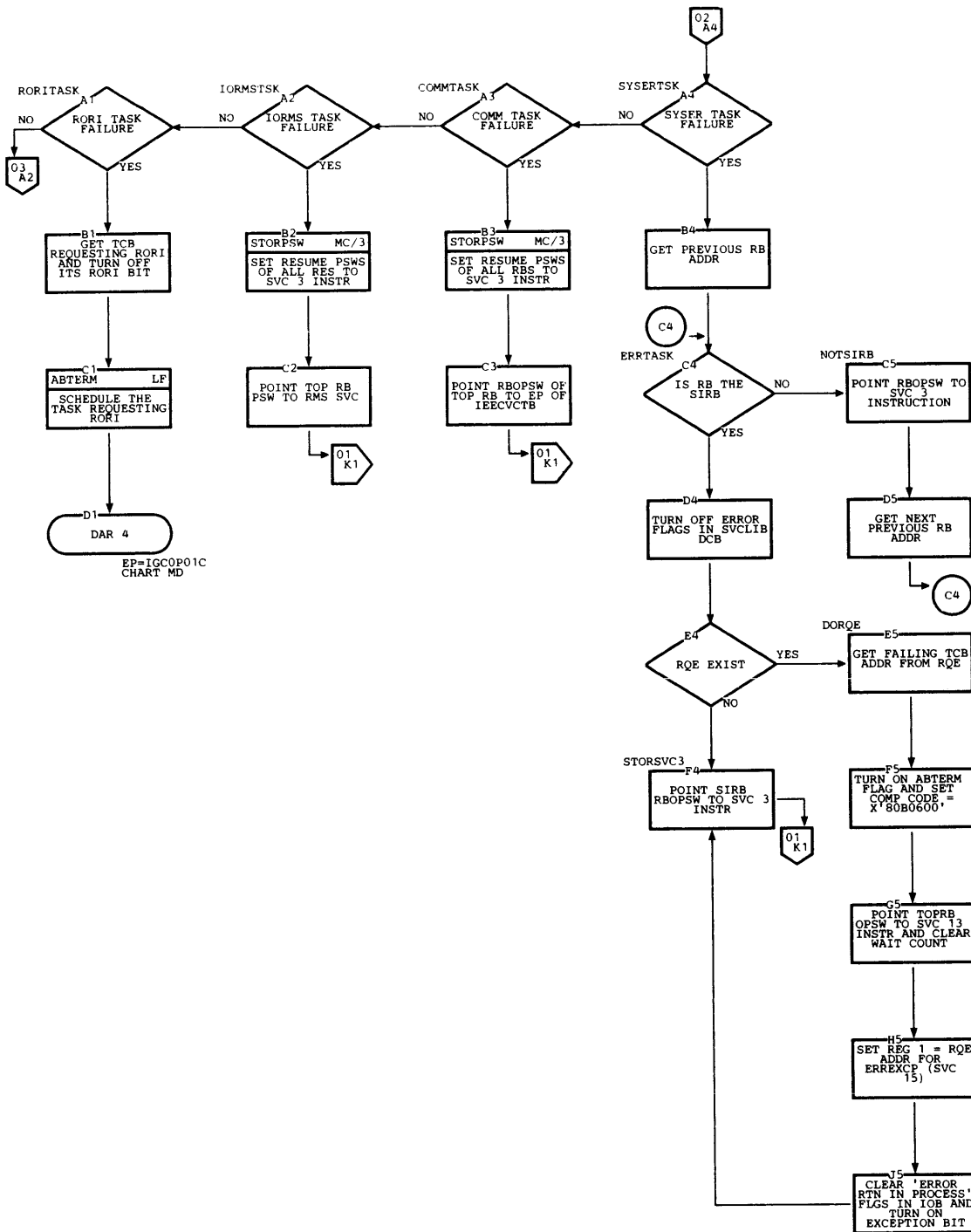
Chart MC. DAR3 (Page 2 of 3)
