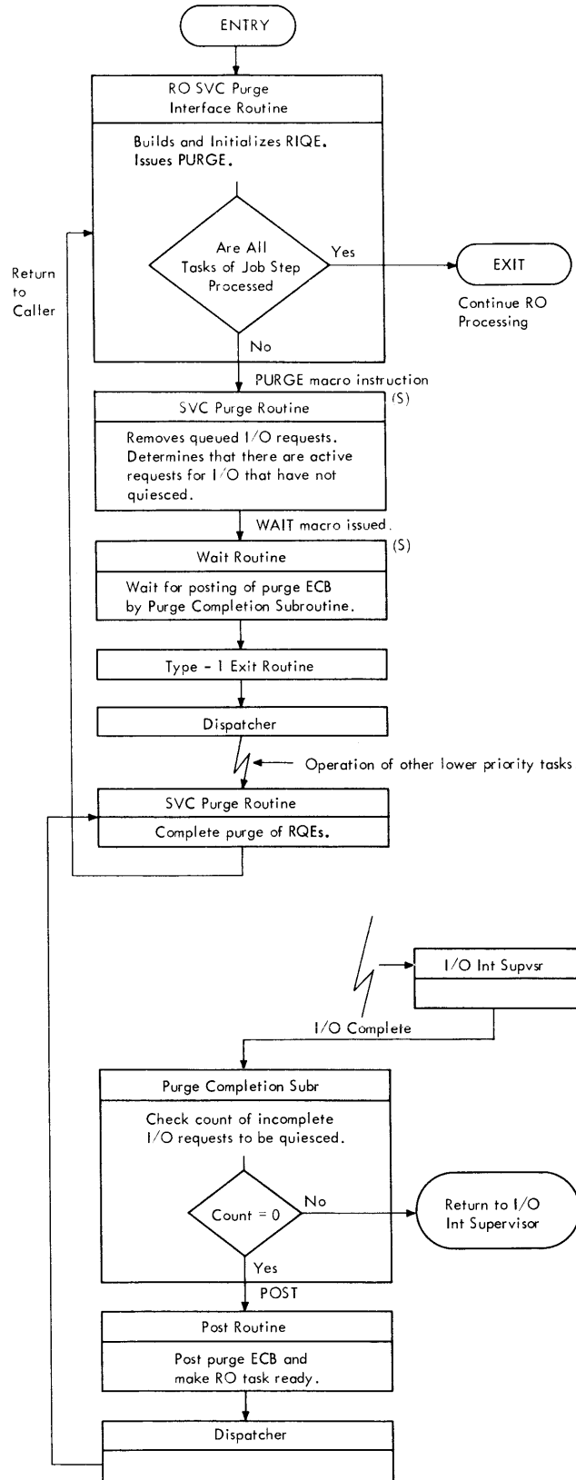
Figure 5-12. Interfaces Between Rollout Module and SVC Purge Routine
