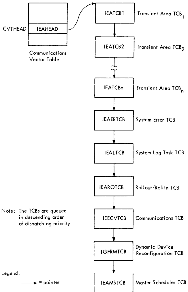
Figure 5-8. Position of Rollout/Rollin TCB on TCB Queue
