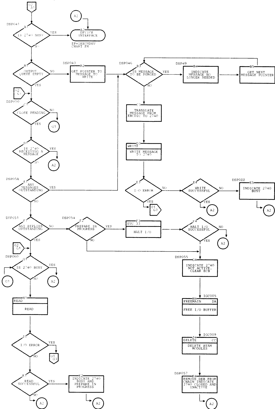
Chart FW. 2740 Processor -- Communications Task with Multiple Console Support (Page 2 of 2)
