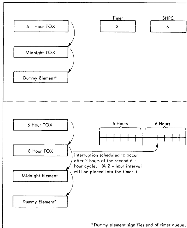
Figure 6-2. Positioning of Elements on the Timer Queue
