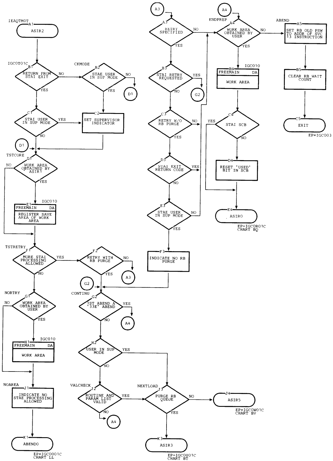
Chart BS. ABEND/STAE Interface 2 Routine (ASIR2)
