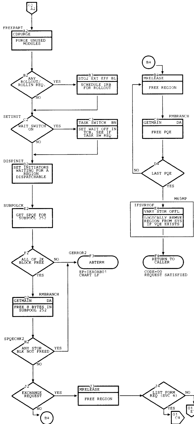
Chart LB. GETPART/FREPART Routine (Page 2 of 2)
