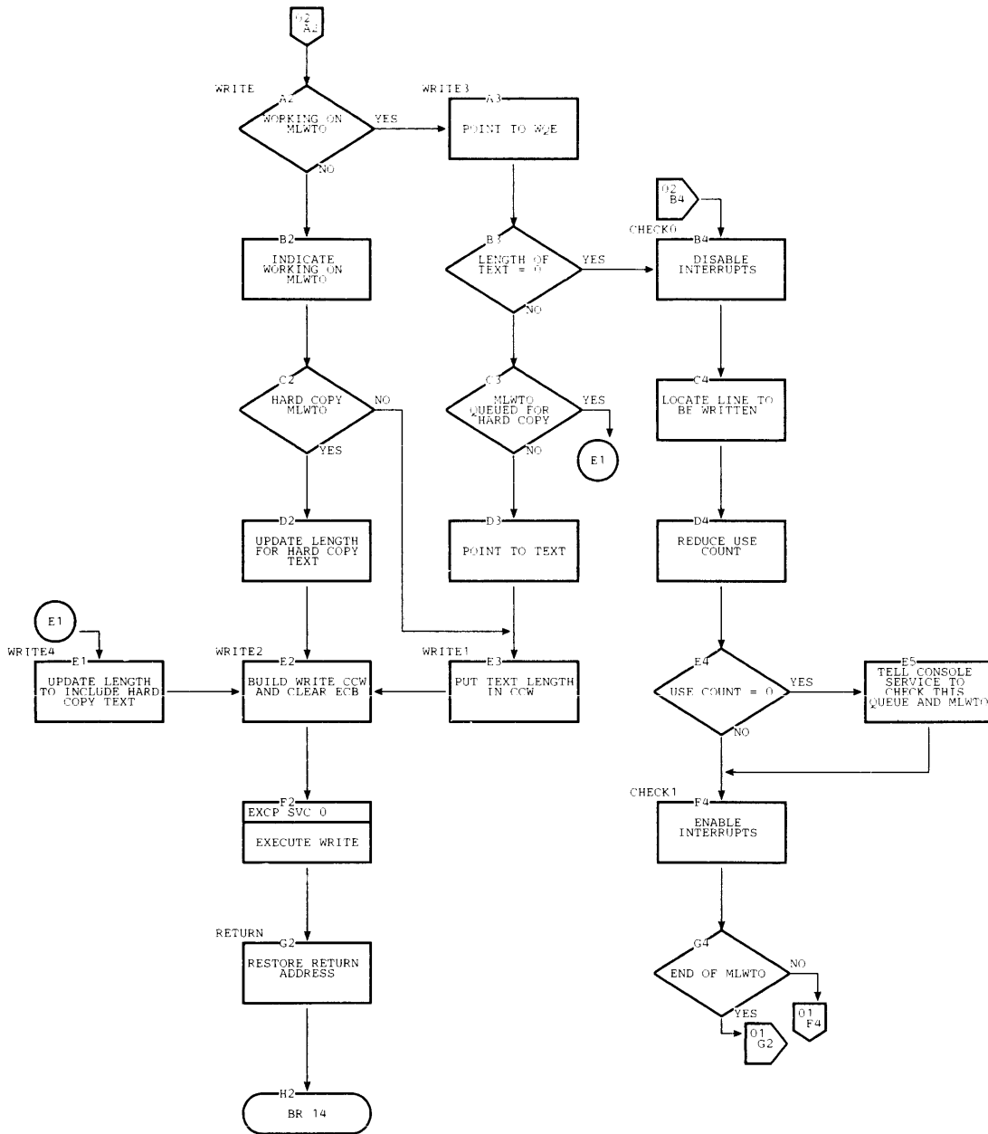
Chart FS. 1052 Processor 2 -- Communications Task with Multiple Console Support (Page 2 of 2)
