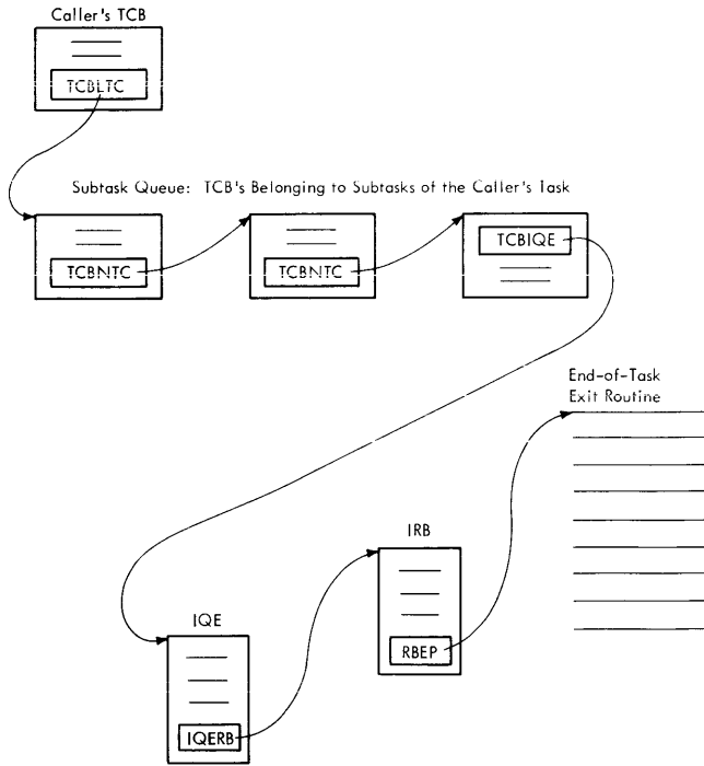
Figure 3-1. Queue Relationships among a TCB, IQE, IRB, and End-Of-Task Exit Routine
