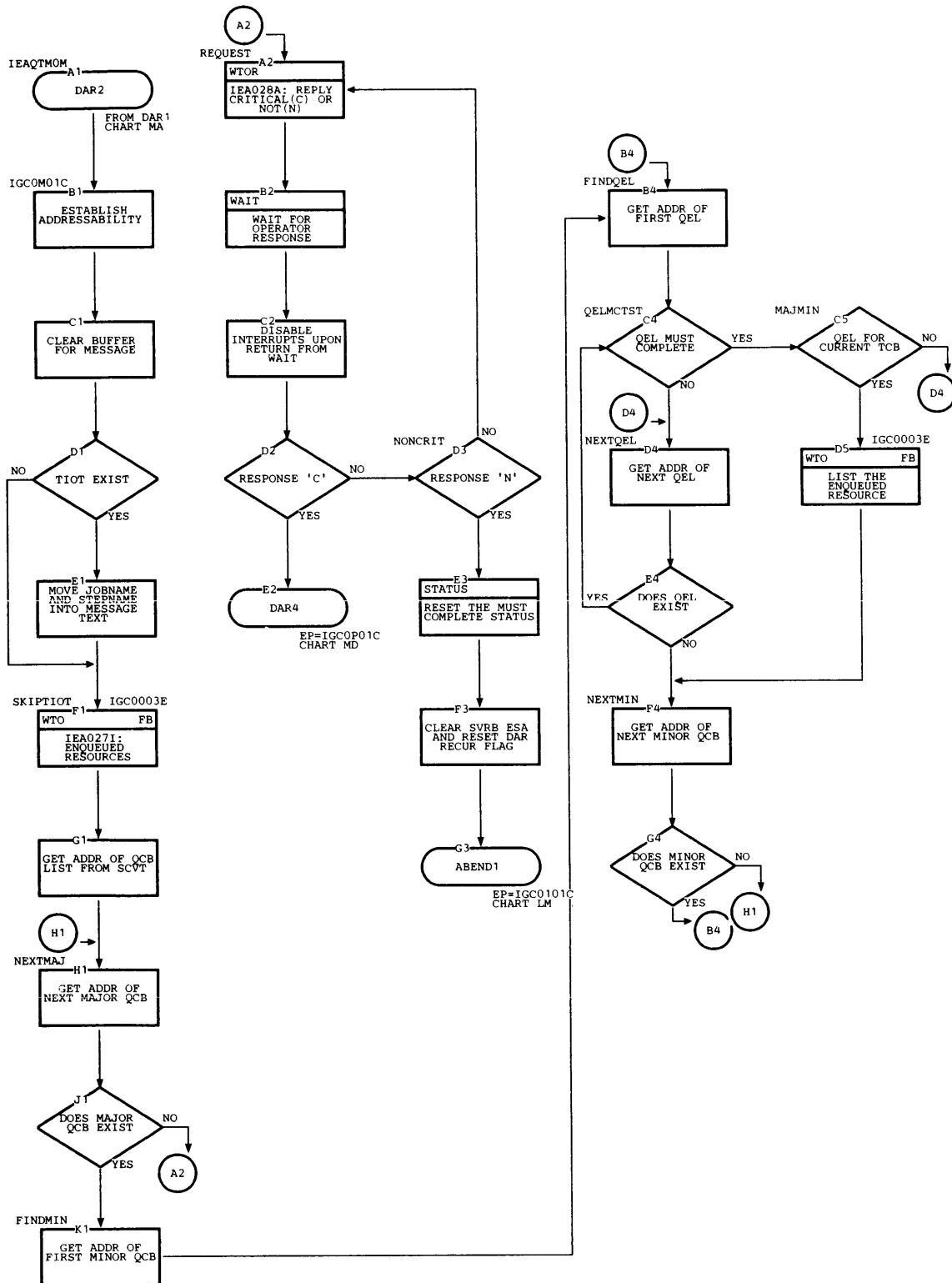
Chart MB. DAR2
