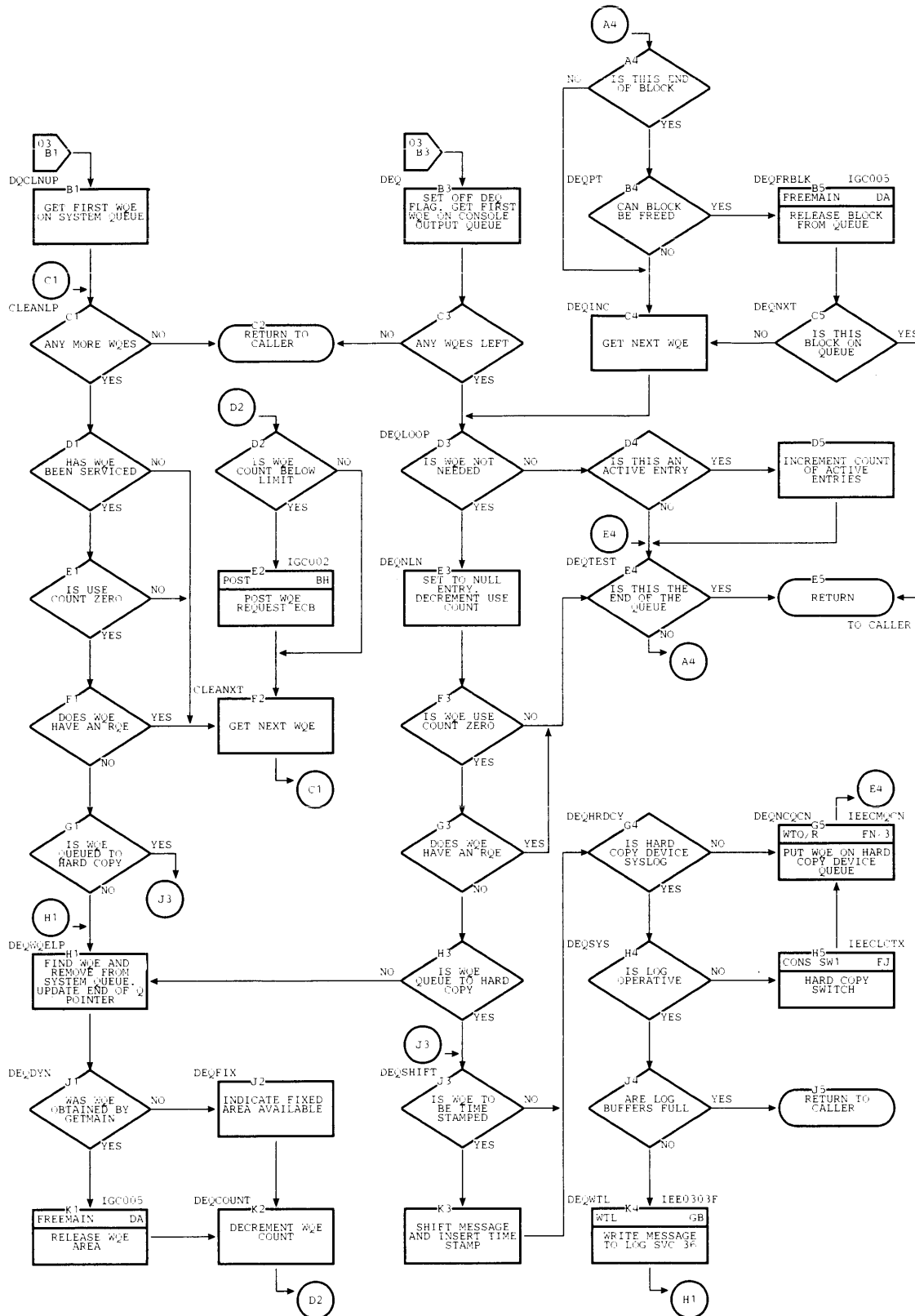
Chart FM. Device Interface -- Communications Task with Multiple Console Support (Page 3 of 3)
