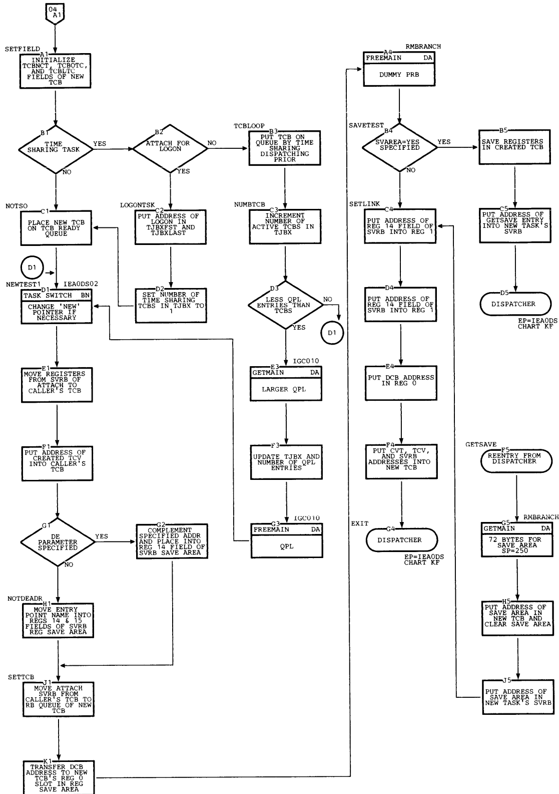
Chart EA. Attach Routine (Page 4 of 4)
