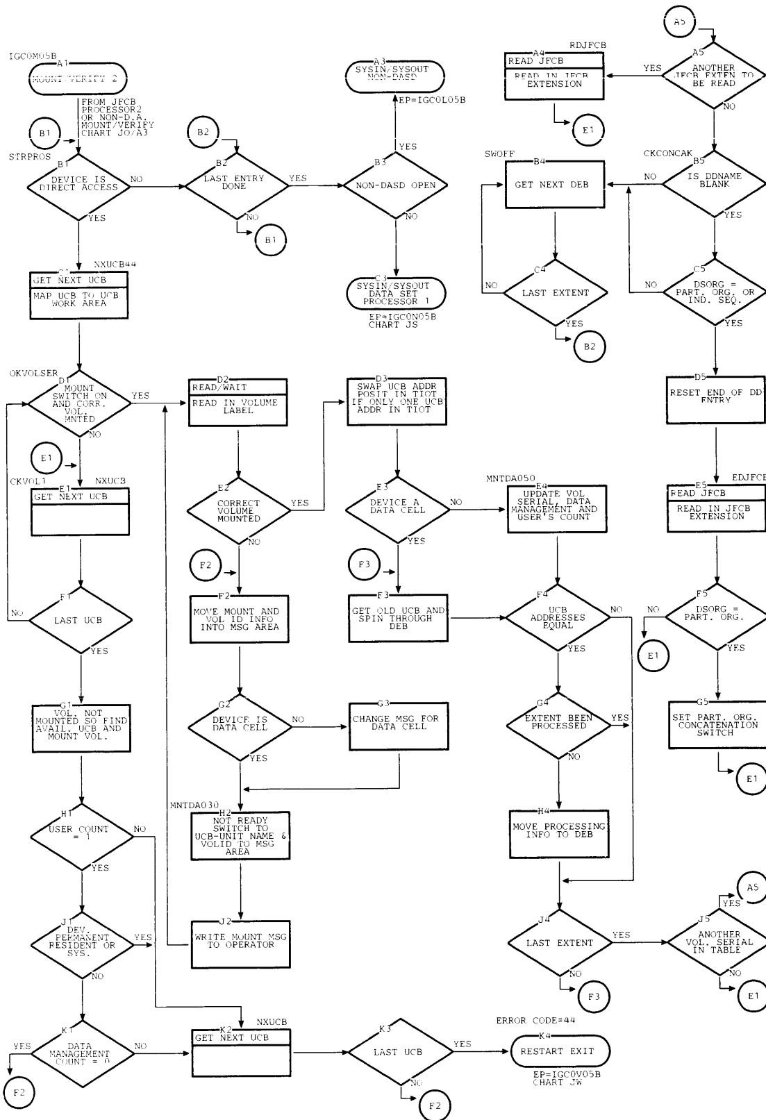
Chart JR. Restart Mount Verify 2 Routine (Direct Access)
