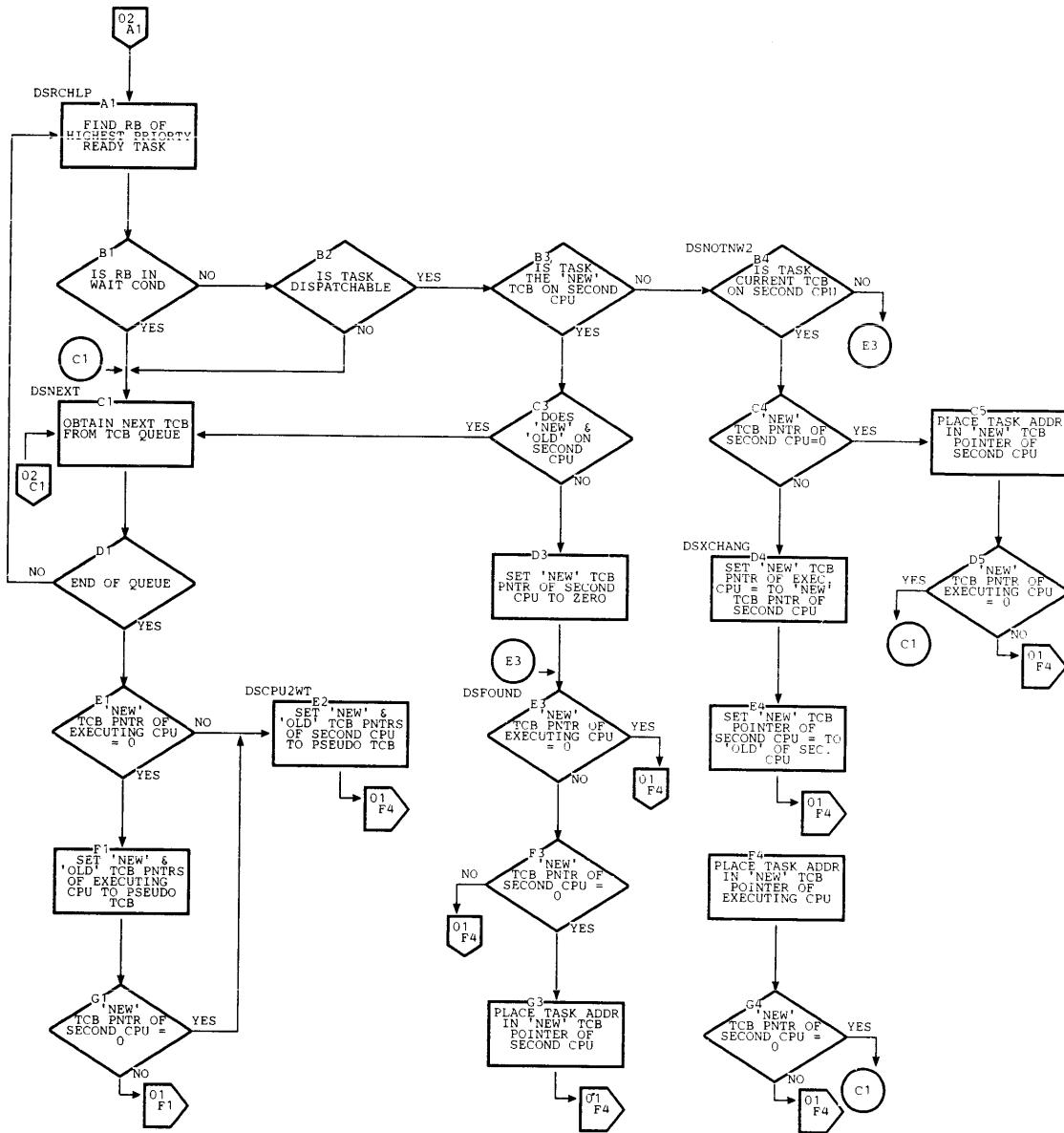
Chart KJ. Dispatcher with Multiprocessing (Page 2 of 2)
