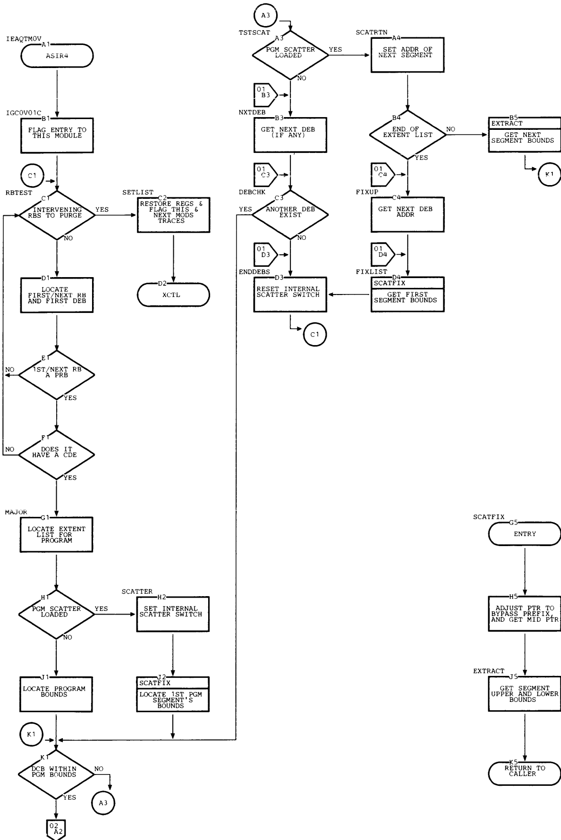
Chart BU. ABEND/STAE Interface 4 Routine (ASIR4) (Page 1 of 4)
