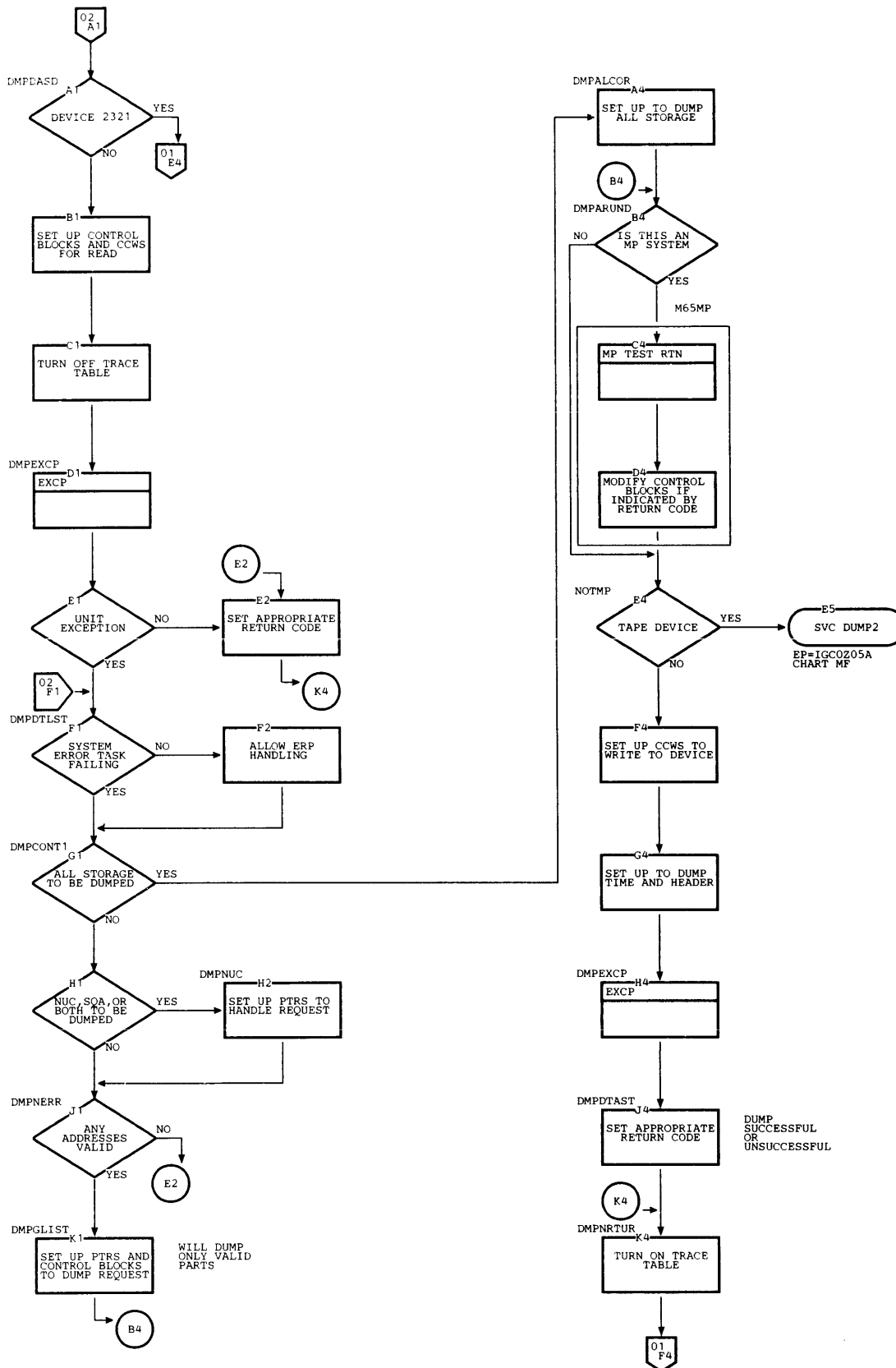
Chart ME. SVC DUMP 1 (Page 2 of 2)
