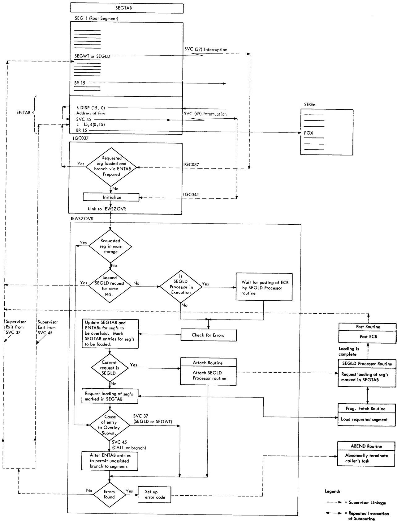
Figure 4-7. Functional Flow of Overlay Supervision
