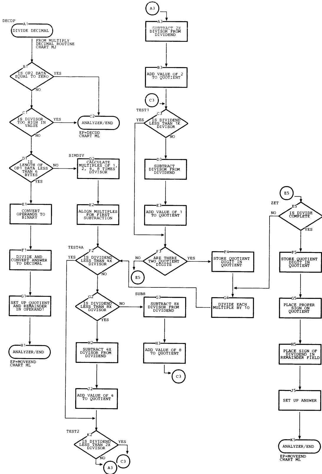
Chart MK. Model 91 Divide Decimal Routine
