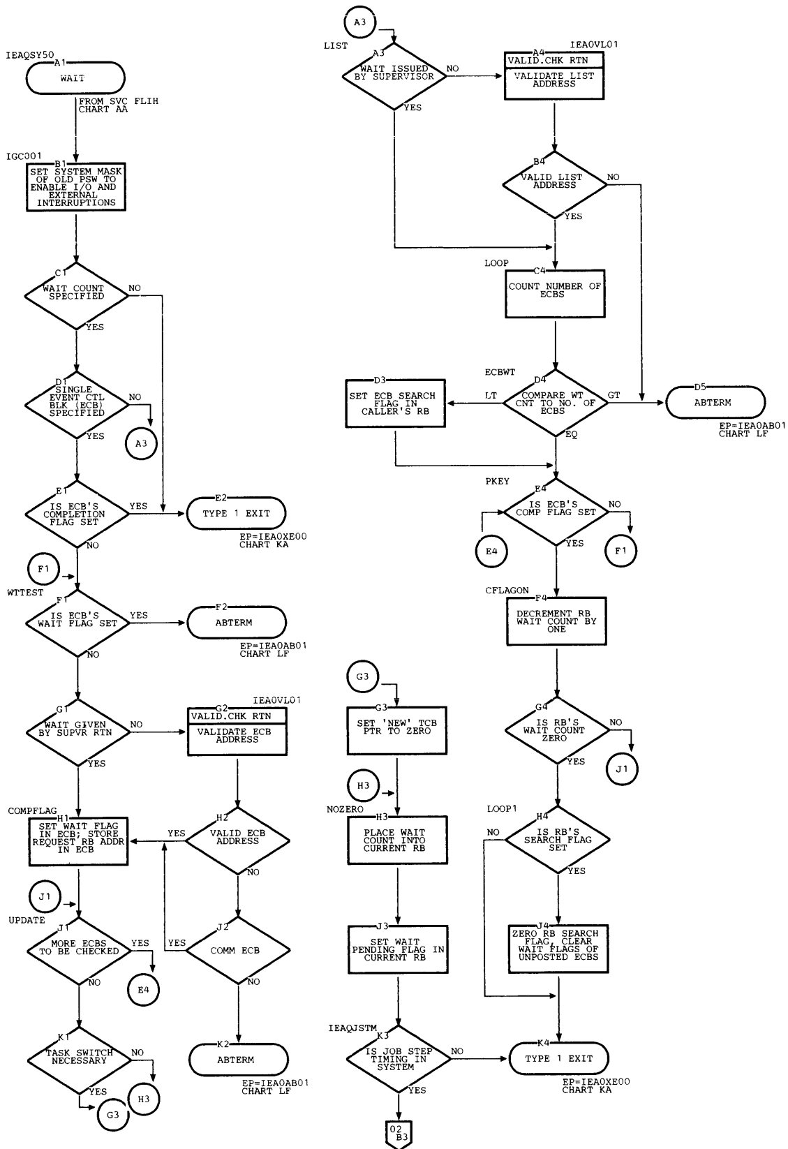
Chart BG. Wait Routine (Page 1 of 2)
