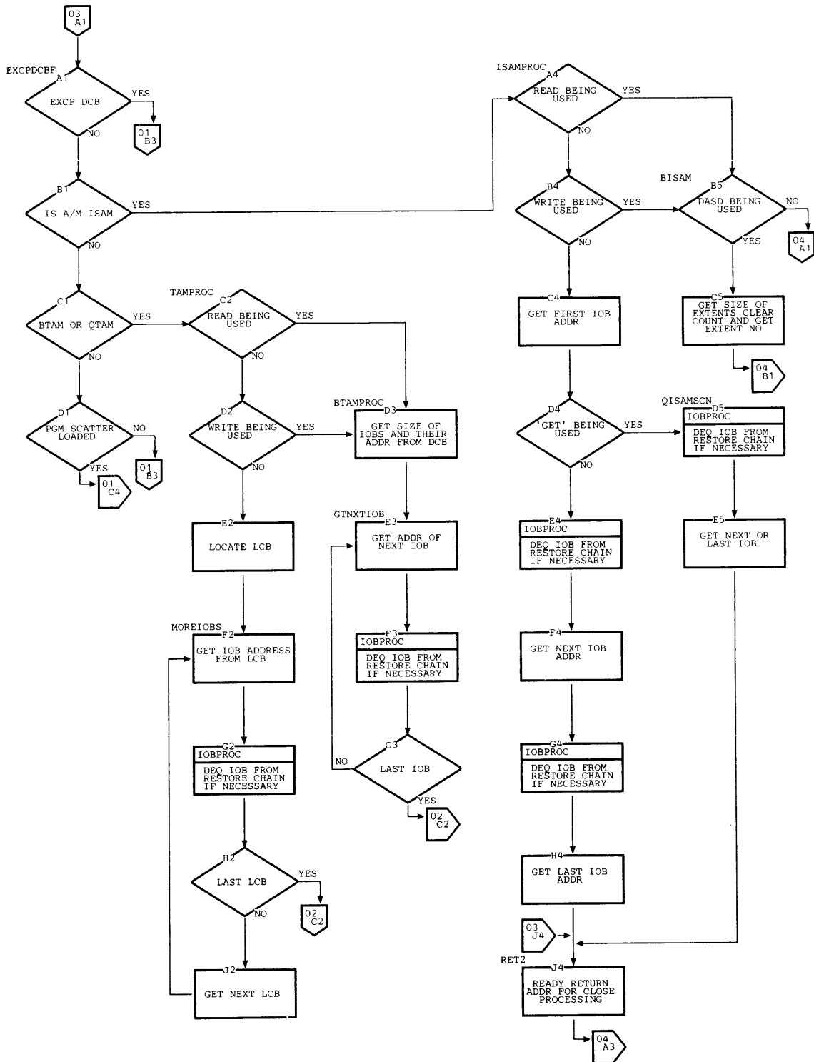
Chart BU. ABEND/STAE Interface 4 Routine (ASIR4) (Page 3 of 4)
