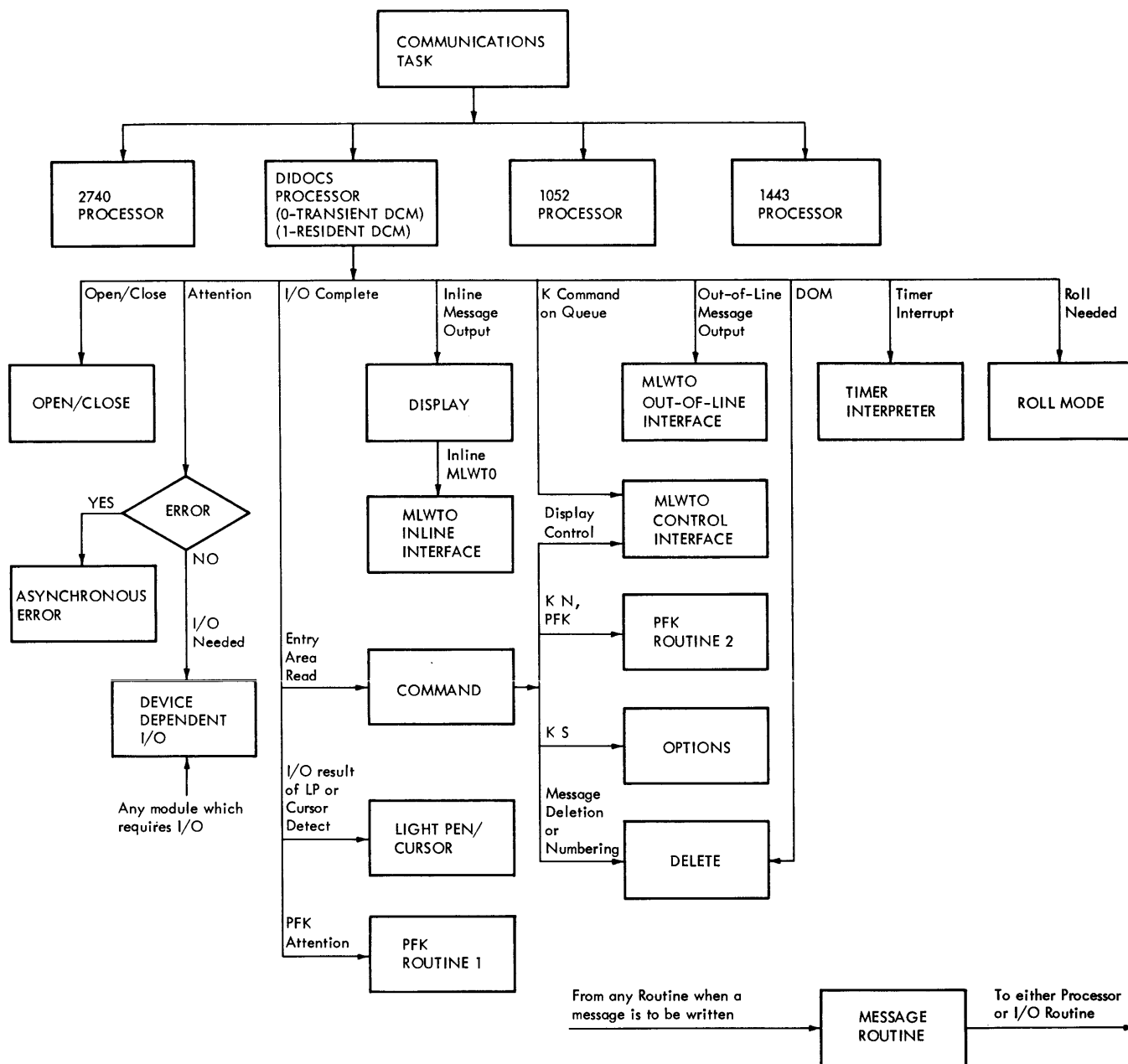
Figure 7-7. CRT Console Support (High Level)
