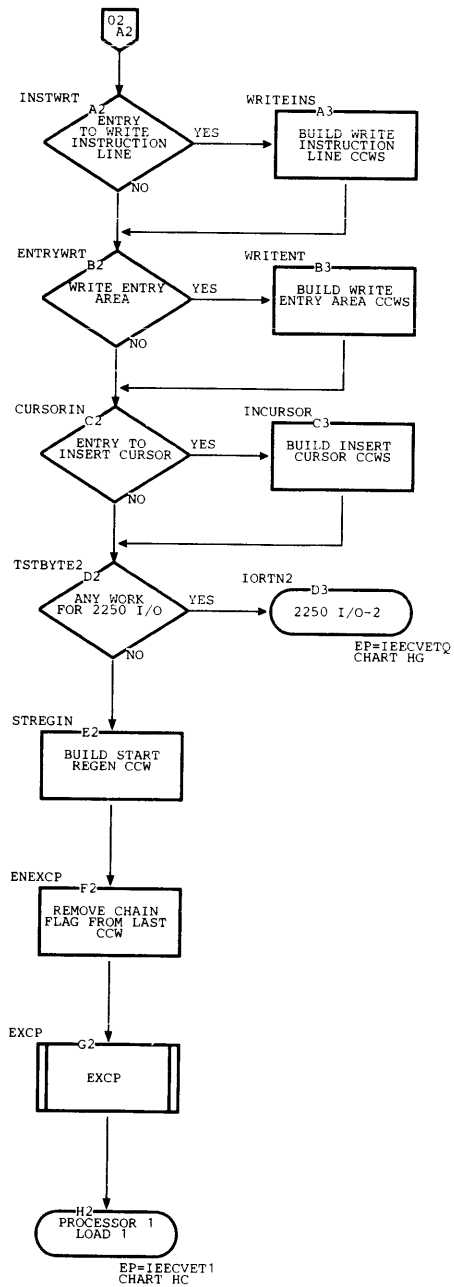
Chart HF. DIDOCS 2250 I/O-1 Routine (Page 2 of 2)
