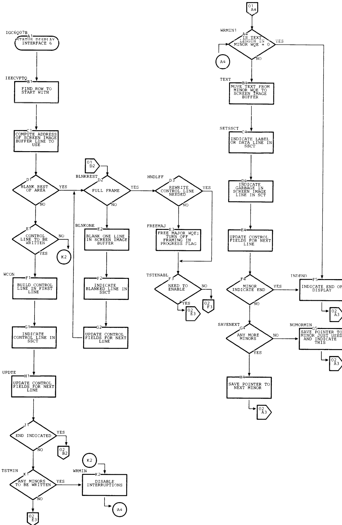
Chart 10. Status Display Interface 6 Routine (Page 1 of 2)
