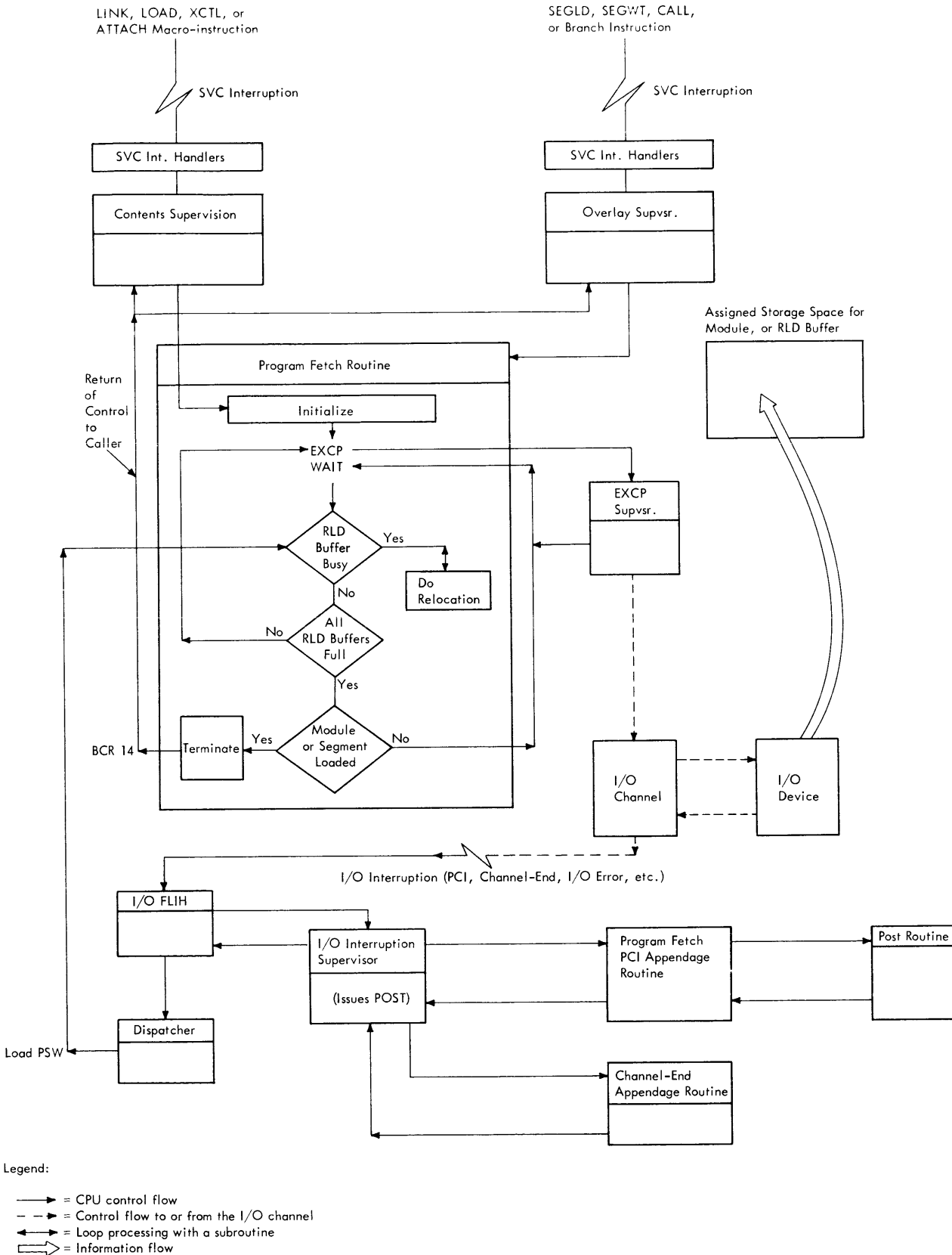
Figure 4-18. Overall Control Flow During the Loading of a Module or Segment
