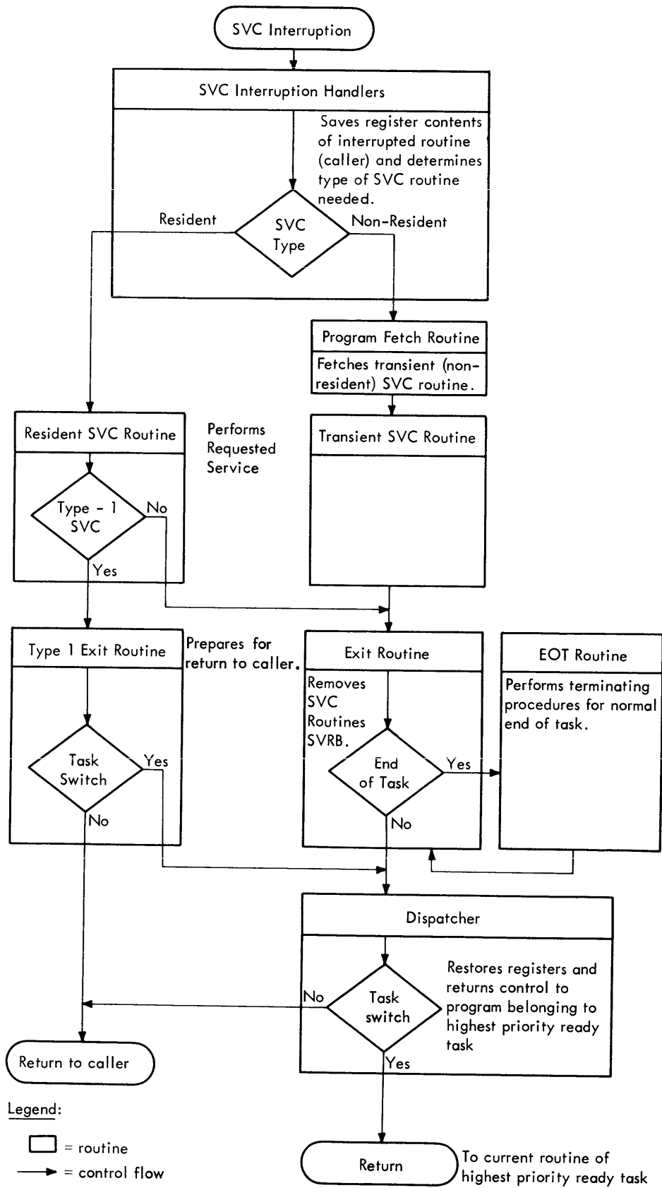
Figure 1-3. Processing After an SVC Interruption
