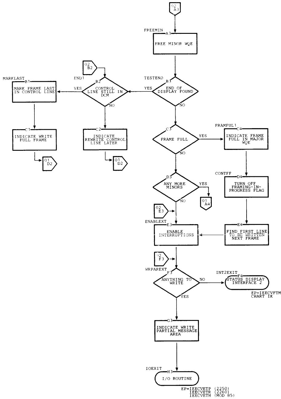
Chart IO. Status Display Interface 6 Routine (Page 2 of 2)
