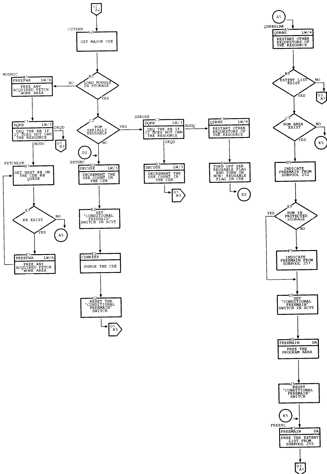
Chart IW. ABEND15 (Page 2 of 5)
