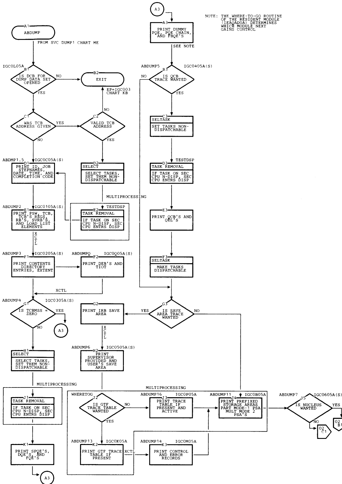
Chart II. ABDUMP Modules (Page 1 of 2)
