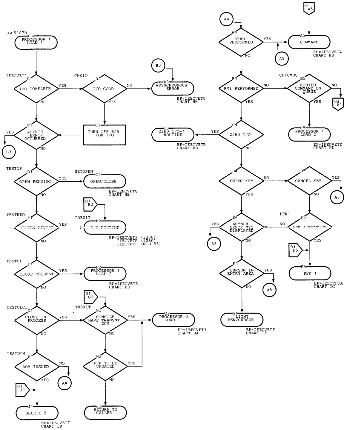
Chart HC. DIDOSCS Processor 1, Load 1 (Page 1 of 2)
