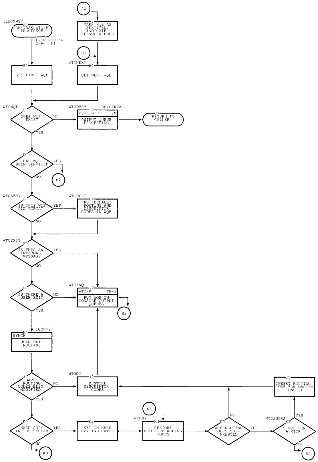
Chart FN. WTO/R Processor -- Communications Task with Multiple Console Support (Page 1 of 3)
