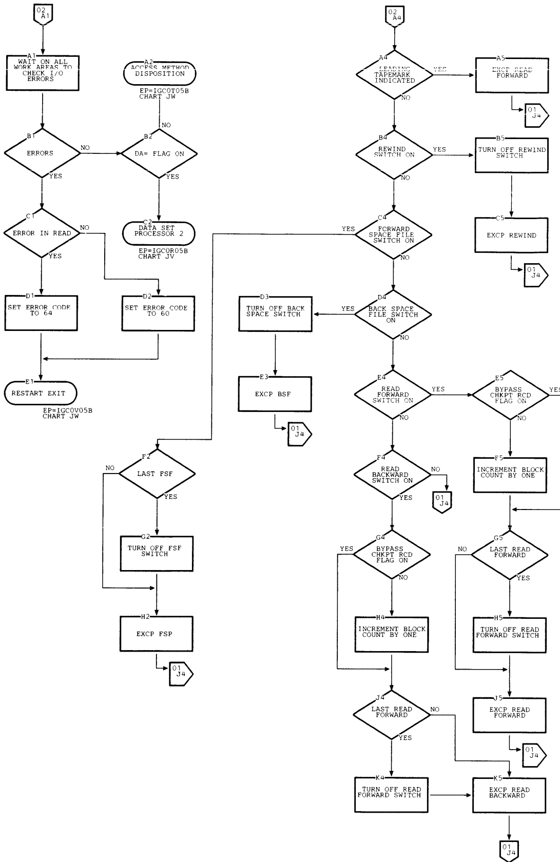
Chart JY. DCS Tape Data Set Processor (Page 2 of 2)
