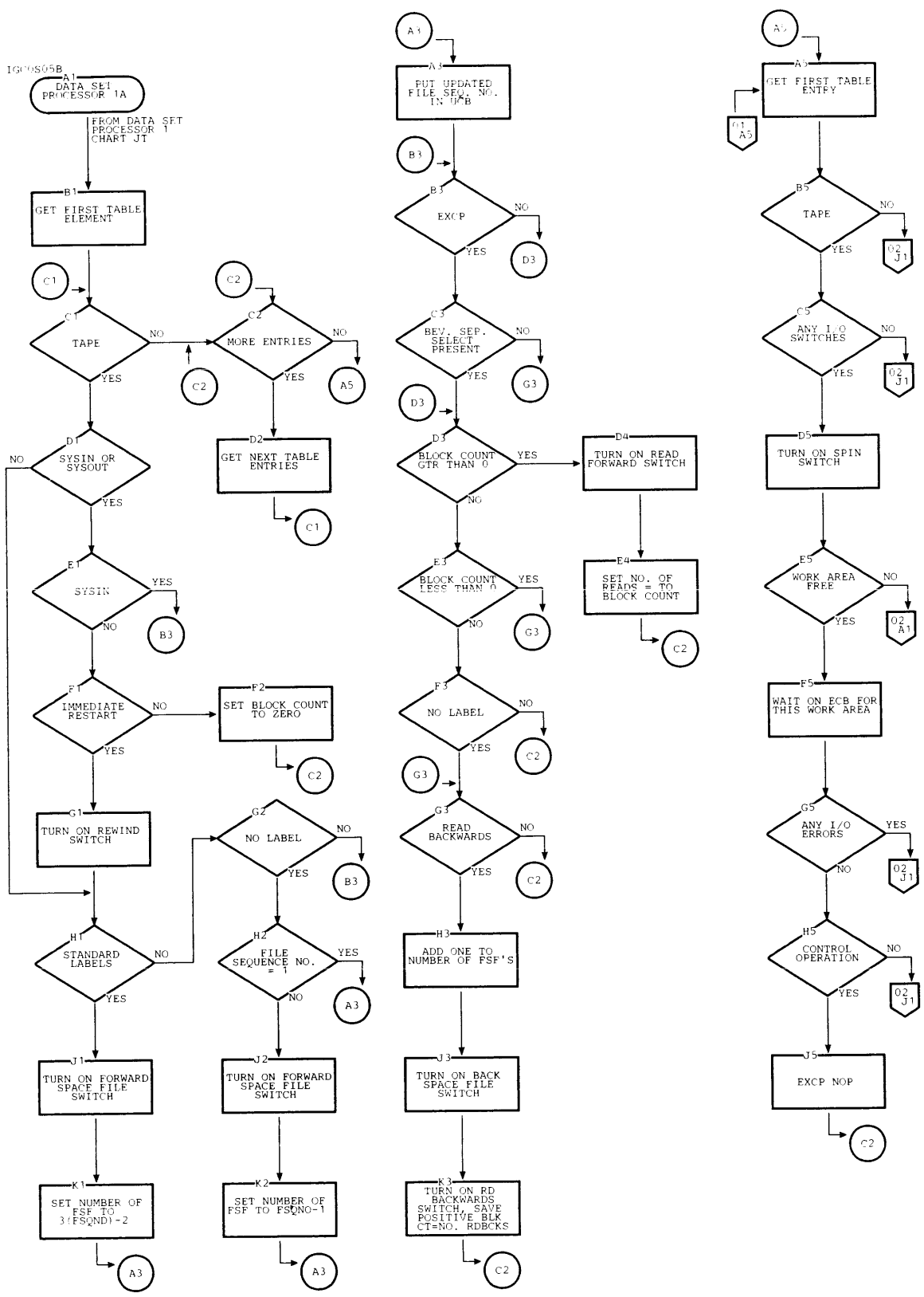
Chart JU. Restart Data Set Processor 1A -- Non-Direct Access (Page 1 of 2)
