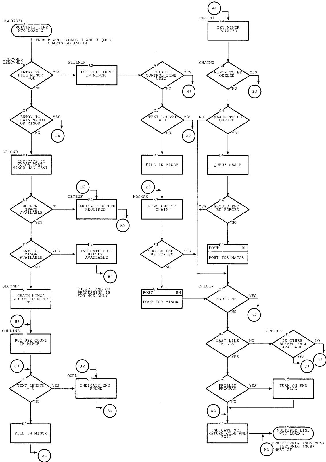
Chart GE. Multiple-Line Write-to-Operator -- Ioad 2
