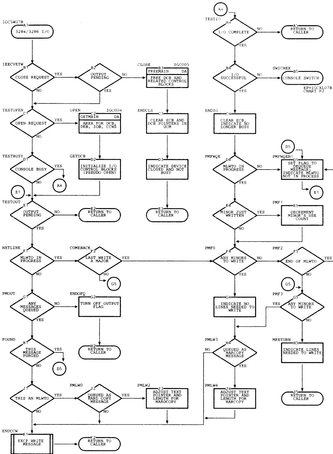
Chart FX. 3284/3286 Processor -- Communications Task with Multiple Console Support
