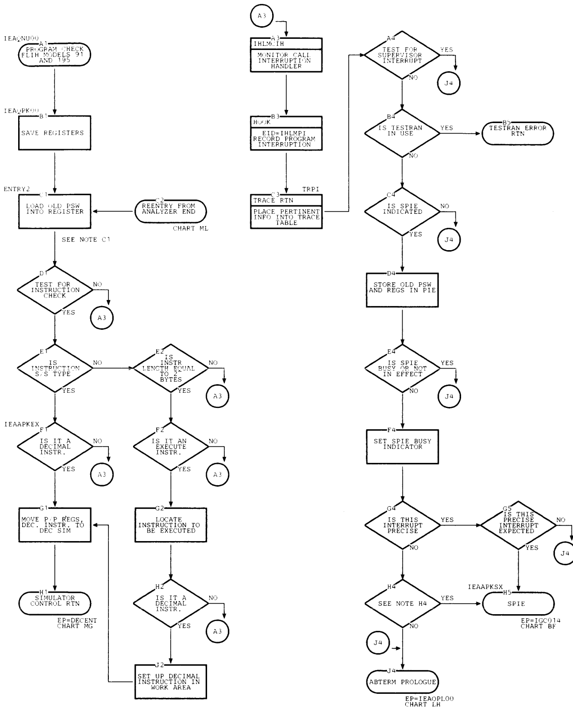
Chart AG. Program Check First-Level Interruption Handler -- Models 91 and 195
