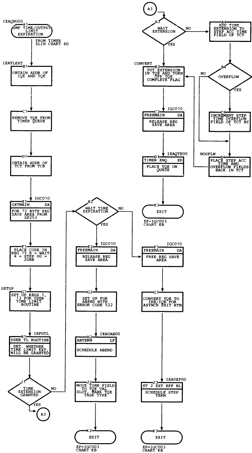
Chart MN. System Management Facility Time/Output Limit Expiration Routine
