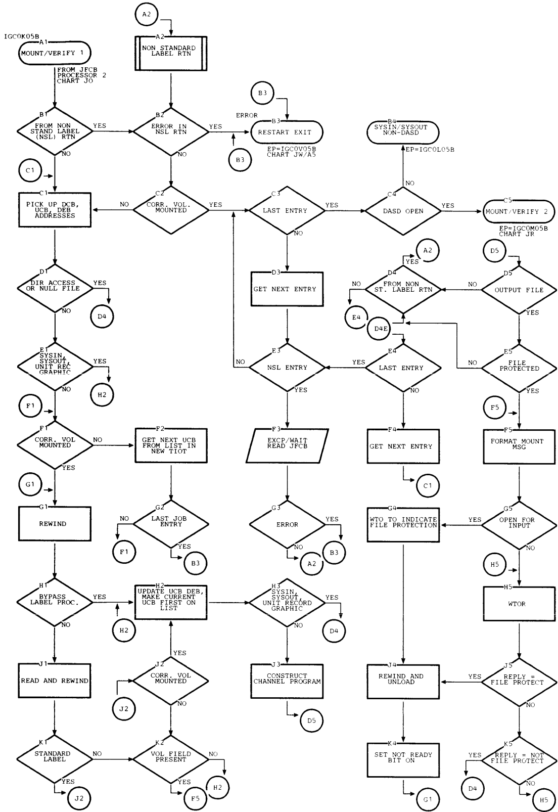
Chart JQ. Restart Mount Verify 1 Routine (Non-Direct Access)
