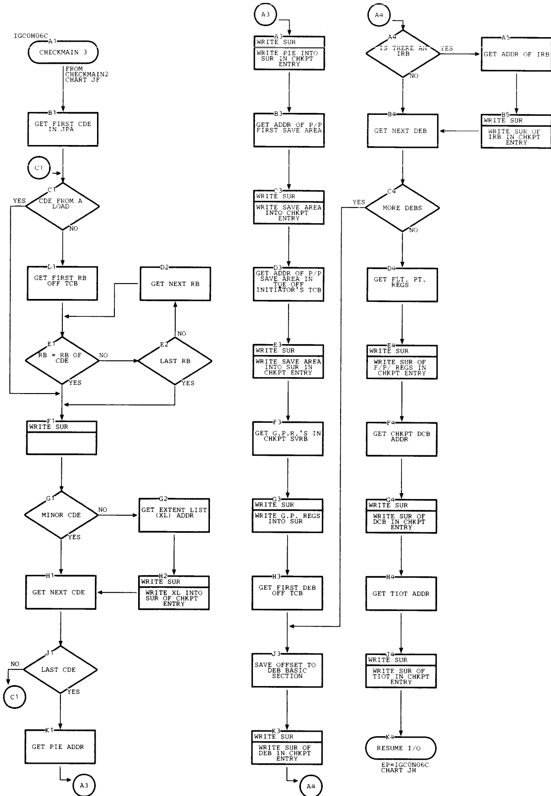
Chart JG. Checkpoint Checkmain 3 Routine
