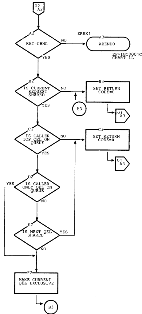
Chart EI. ENQ Routine (Page 2 of 2)
