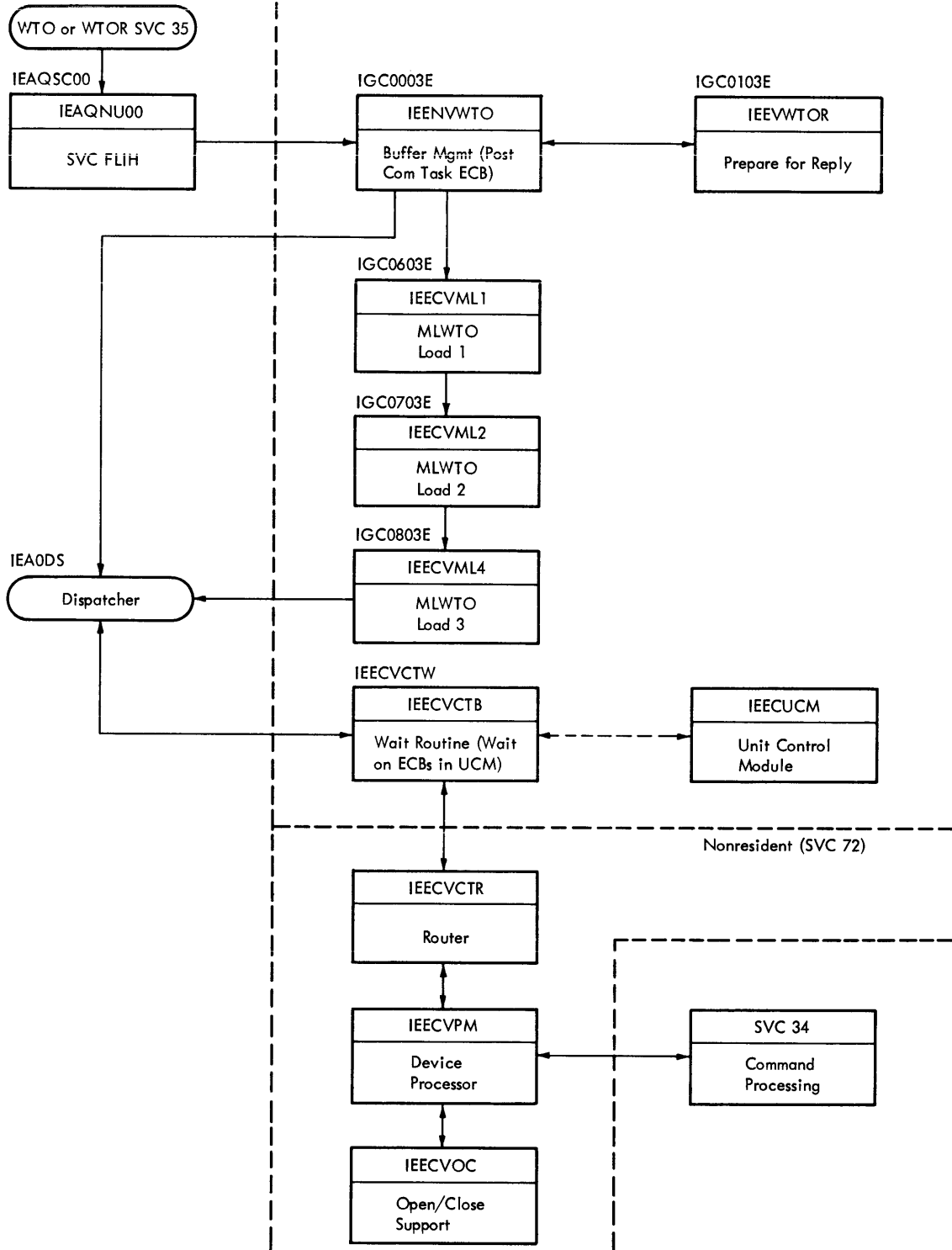
Figure 7-2. Console Support: Output
